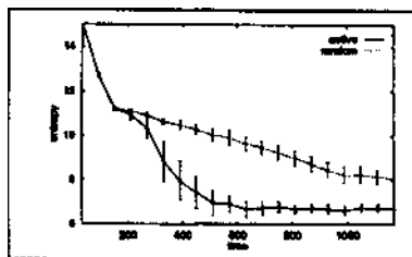
Fig. 11. Entropy of belief states
