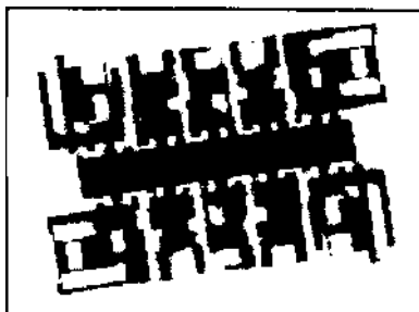
Fig. 8. E_\alpha[H] + v(\alpha) at pos. 3
