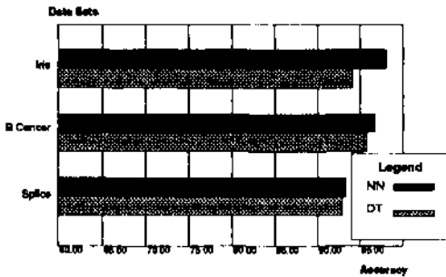
Figure 2: Comparison: predictive accuracy for the three datasets.
