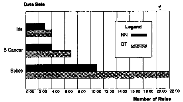
Figure 4: Comparison: number of rules for the three datasets.
