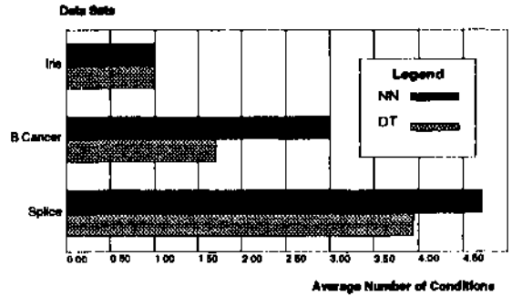
Figure 3: Comparison: average number of a rule's conditions for the three datasets.
