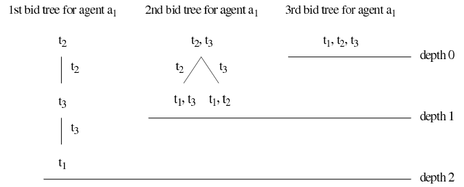
Figure 3: Bid Trees for SSI Auctions with Bundle Size Three
