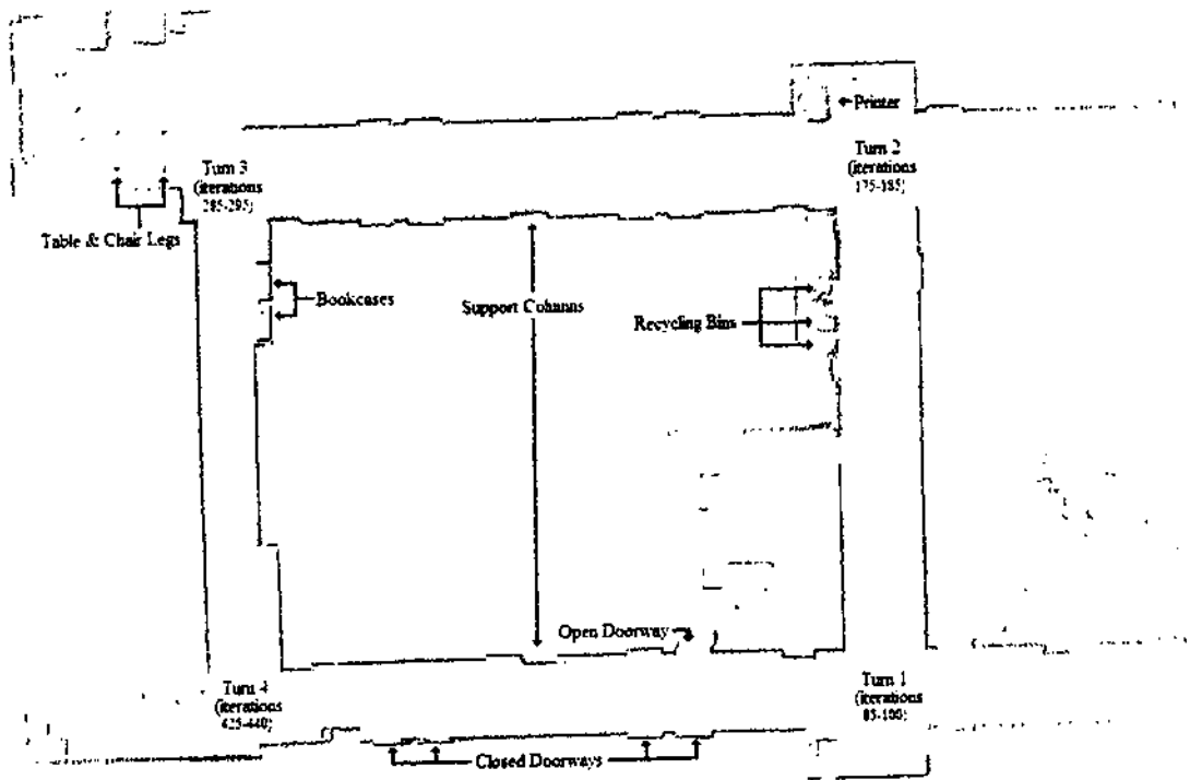
Figure 1: A DP-SLAM map with 9000 particles.
