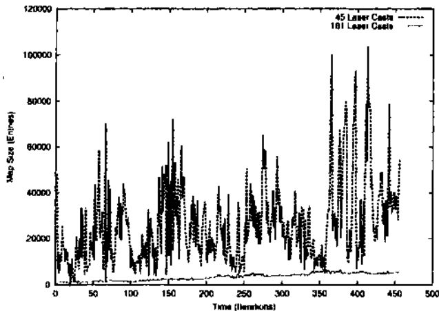
Figure 4: Total map entries used over time.
