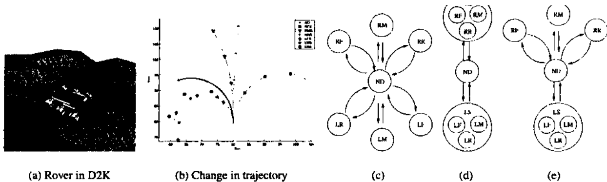
Figure 2: (a) Snapshot from the dynamic simulation of the six wheel rocker bogie rover in the simulator, (b) An example showing the normal trajectory (ND) and the change in the same trajectory with a fault at each wheel, (c) Original discrete state transition model. The discrete states are: Normal driving (ND), right and left, front, middle and rear wheel faulty (RF, RM, RR, LF, LM, LR) (d) Abstract discrete state transition model. The states, RF, RM and RR have been aggregated into the Right Side wheel faulty states and similarly LF, LM and LR into Left Side wheel faulty states (RS and LS). (e) State space model where RS has been refined. All states have self transitions that have been excluded for clarity.
