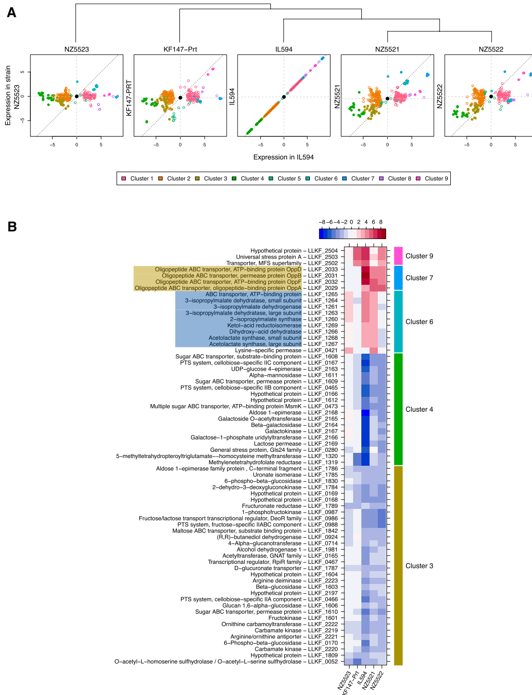
Figure 2. Genome-wide gene expression profiles during exponential growth in milk. All strains are compared to the wild-type strain KF147, and \log_2 -transformed expression ratios are displayed. (A) Expression levels of all differentially regulated genes compared to KF147 ( p < 0.001 in at least one of the strains) in relation to that of the dairy isolate IL594. Genes that are not differentially expressed with respect to strain KF147 map on the center of the plot (●). Expression levels of genes falling either in the bottom left or the top right quadrant show transcript changes toward the levels found in IL594. Genes falling in the top left or bottom right quadrant show changes in the opposite direction compared with IL594. Transcript levels similar to those found in the dairy isolate are identified as dots close to the diagonal of the plot (dotted line). The tree at the top of panel A summarizes the similarity of gene expression between the strains. (B) The differential gene expression in detail for the five most discriminating clusters. Only genes of clusters with an average differential expression of at least fourfold in at least one of the three evolved strains are plotted (corresponding to solid symbols in panel A). Gene functional annotations and identifiers are listed. Brown and blue shading indicates genes/putative operons containing point mutations in the upstream promoter region in at least one of the adapted strains. The heat map on the top of panel B displays the \log_2 -transformed differential expression levels.
