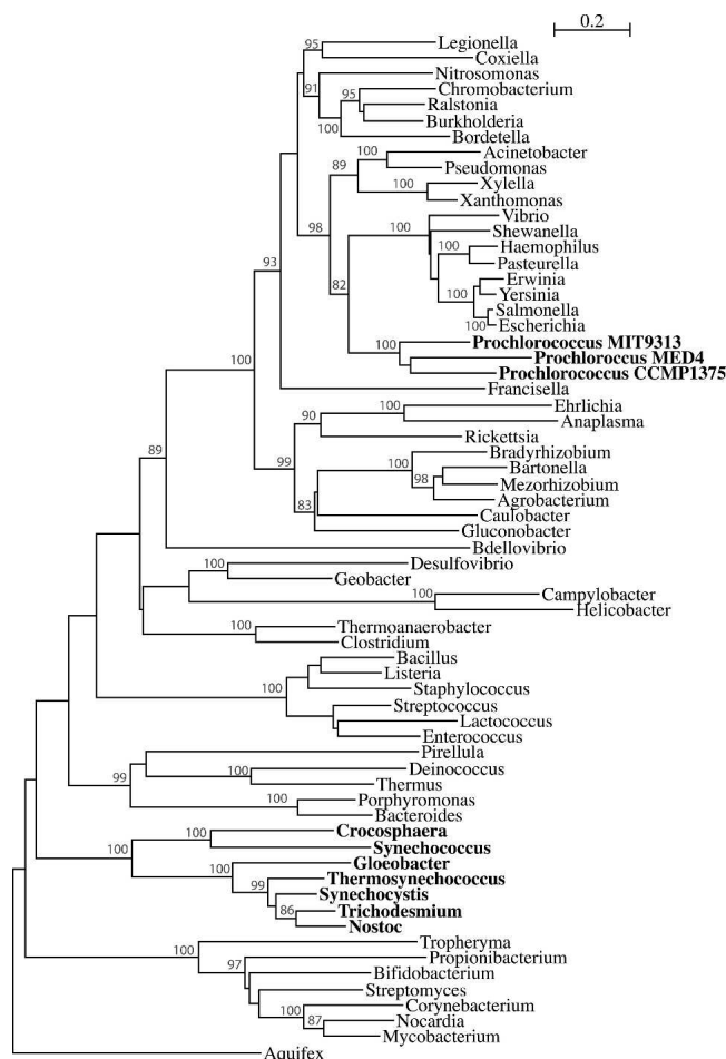
Figure 5. Example of horizontal gene transfer to cyanobacteria: threonyl tRNA synthetase. This is a phylogenetic tree reconstructed from a data set in which the Anabaena sp. genome did not have a detectable homolog in its annotation. In this tree, sequences of three Prochlorococcus spp. group within Gamma-proteobacteria with high bootstrap support. The presence of an ancestrally transferred gene constitutes a shared derived character for the descendants (Andersson et al. 2005; Huang et al. 2005), suggesting that the three Prochlorococcus spp. form a monophyletic group. Note that despite coherency of the remaining cyanobacteria as a group, the relationships within cyanobacteria do not follow the plurality topology. tRNA synthetases are known to have complex evolutionary histories involving multiple HGT events (e.g., Wolf et al. 1999). Cyanobacteria are shown in bold. To obtain bootstrap support values, a consensus tree was generated from 100 bootstrap sampled trees (see Methods for more details). Only bootstrap support values above 80% are shown. Additional examples of interphylum transfers are available in the Supplemental material.
