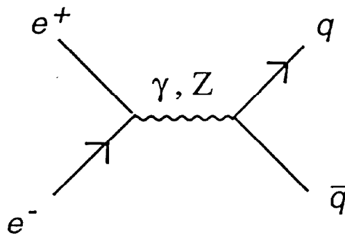
Figure 10: Born diagrams for e^+e^- annihilation.
