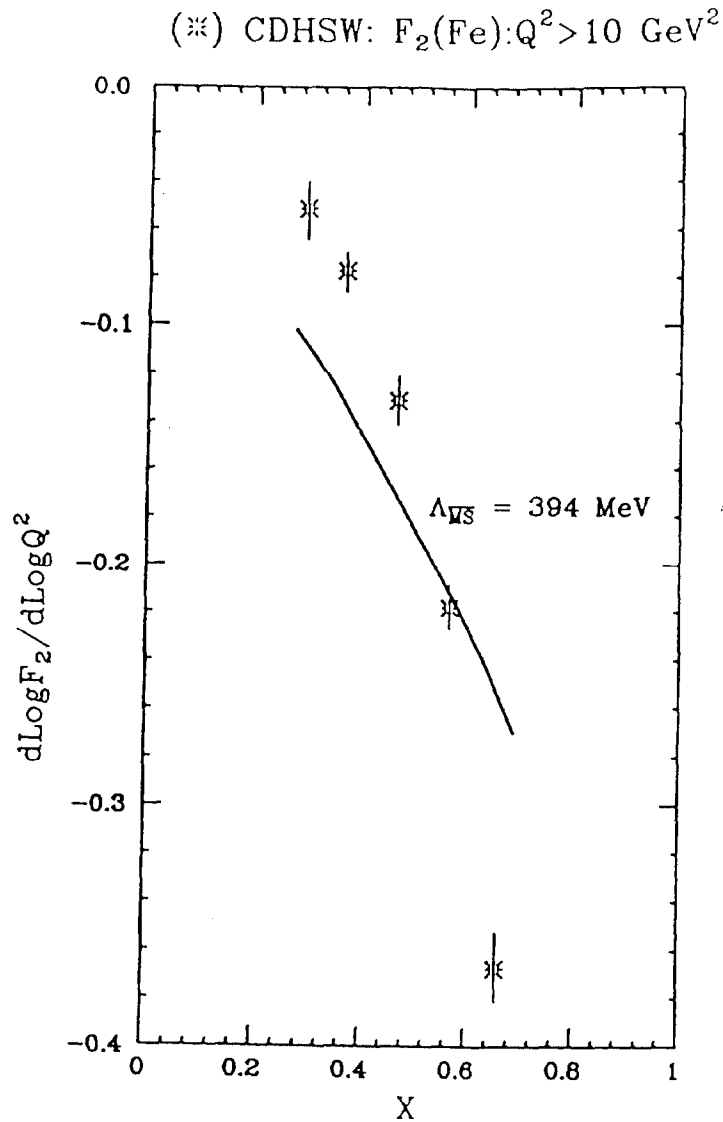
Figure 28: The CDHSW measurement (Berge et al. , 1991) of the logarithmic derivative of F_2 with respect to Q^2 , d\text{Log}F_2/d\text{Log}Q^2 , as a function of x with an iron target. The NLO QCD curve with typical value of \Lambda_{QCD} as analyzed by the BCDMS collaboration (BCDMS Collaboration, 1987b) is also shown.
