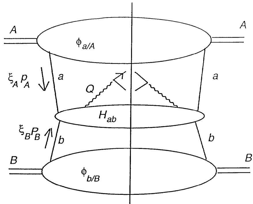
Figure 12: Factorization theorem for Drell-Yan cross section.
