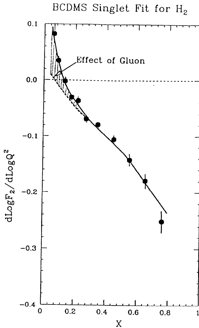
Figure 26: The singlet evolution of the BCDMS (BCDMS Collaboration, 1987a; BCDMS Collaboration, 1987b) measurement of F_2 in a hydrogen target. The effect of gluons, prominent at low x , is shown by the hatched region between the singlet (solid), and non-singlet (dotted) QCD fits. The figure is from (Mishra and Sciulli, 1989).
