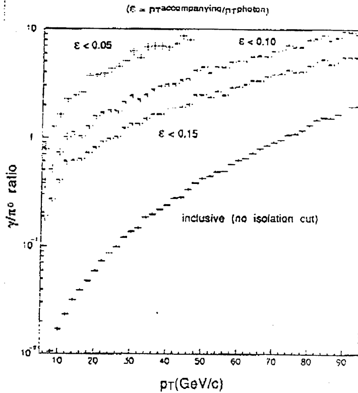
Figure 41: Leading log predictions for \gamma/\pi^0 ratios with various isolation cuts (Bailey and Owens, 1993)
