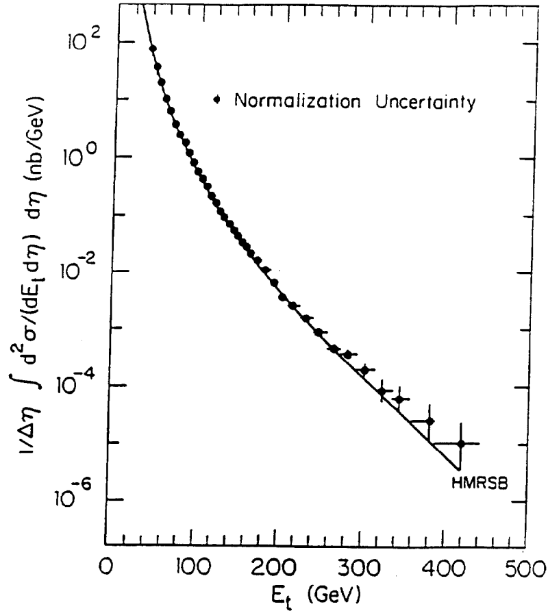
Figure 46: The inclusive jet cross section measured by CDF for a cone size R=0.7 averaged over the pseudorapidity interval 0.1 < \eta < 0.7 . The curve represents the prediction of a NLO calculation using the HMRSB parton distributions. The errors shown represent the statistical and E_t dependent systematic errors. The overall normalization uncertainty is also indicated separately.
