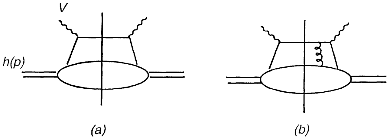
Figure 7: Deeply Inelastic Scattering.
