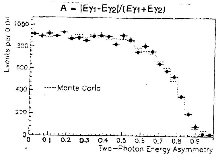
Figure 38: Photon energy asymmetry distribution in \pi^0 decay (Alverson et al. 1992)
