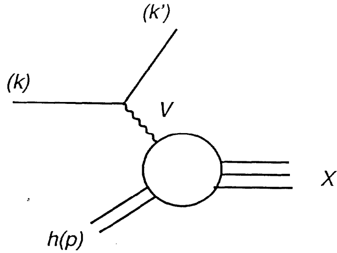
Figure 7: Deeply Inelastic Scattering.
