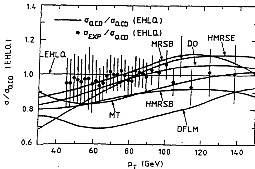
Figure 45: The ratio of experimental to theoretical (based on EHLQ) jet cross section at \eta < 0.85 in the UA2 experiment (black dots). The curves represent calculations for different parton distributions, relative to the EHLQ distributions
