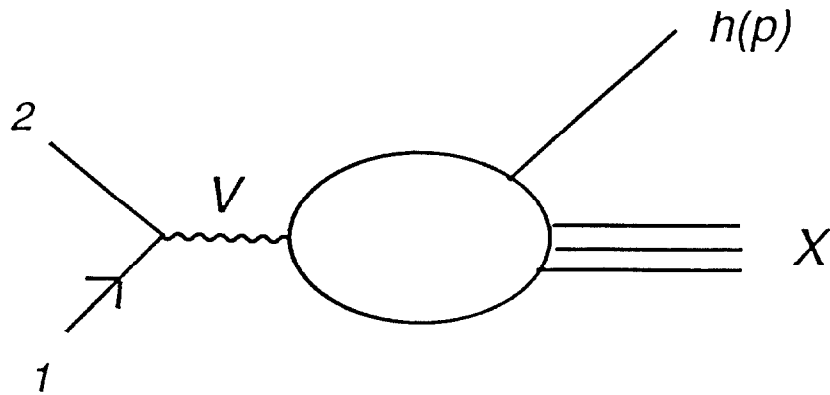
Figure 10: Born diagrams for e^+e^- annihilation.
