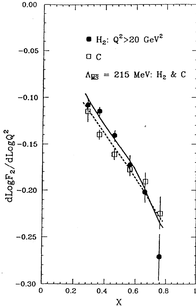
Figure 25: The BCDMS (BCDMS Collaboration, 1987a; BCDMS Collaboration, 1987b) measurement of the logarithmic derivative of F_2 with respect to Q^2 , d\text{Log}F_2/d\text{Log}Q^2 , as a function of x with hydrogen (solid symbols) and carbon (open symbols). The best NLO QCD non-singlet fits to these data are also shown. It is assumed that for x > 0.25 the F_2 data essentially evolve as non-singlets. The figure is from (Mishra and Sciulli, 1989).
