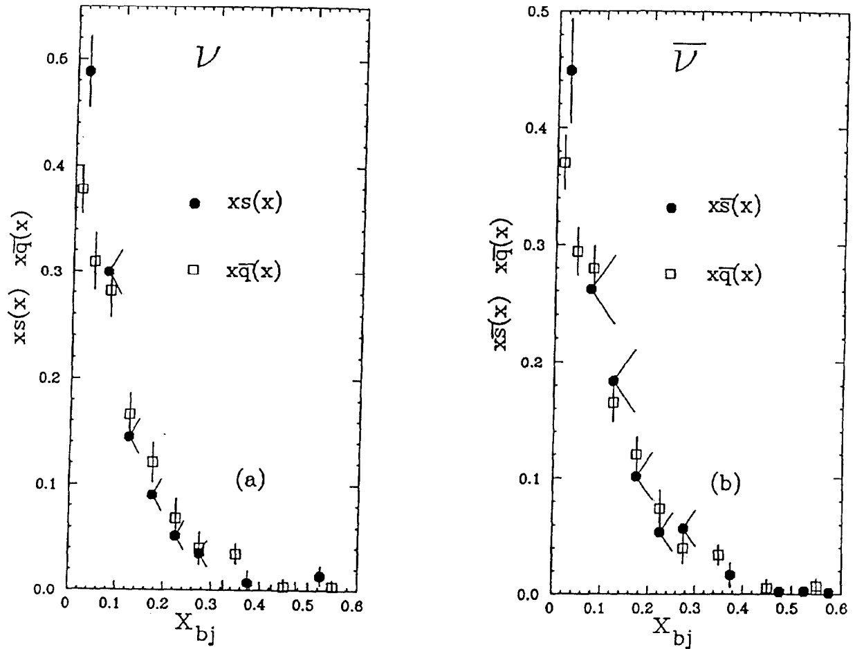
Figure 21: The strange sea component of the nucleon measured (Foudas et al. , 1990) by analyzing the CCFR \nu_{\mu} - and \bar{\nu}_{\mu} -induced opposite sign dimuons. The s(x) and \bar{s}(x) are compared to the non-strange \bar{q}(x) obtained from ordinary single muon events. To illustrate the “shape-difference”, the total \bar{q}(x) are normalized to the respective strange sea distribution.
