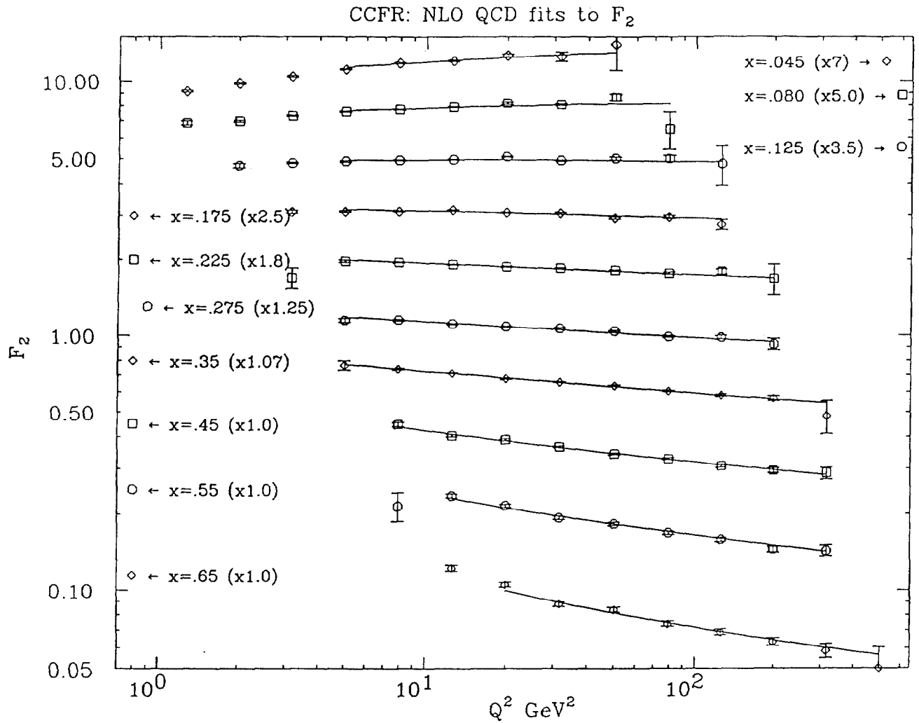
Figure 29: The F_2 data of CCFR (Quintas et al. , 1993) and the best NLO QCD fit. Cuts of Q^2 > 5 \text{ (GeV/c)}^2 and x < 0.7 were applied for a next-to-leading order fit including target mass corrections.
