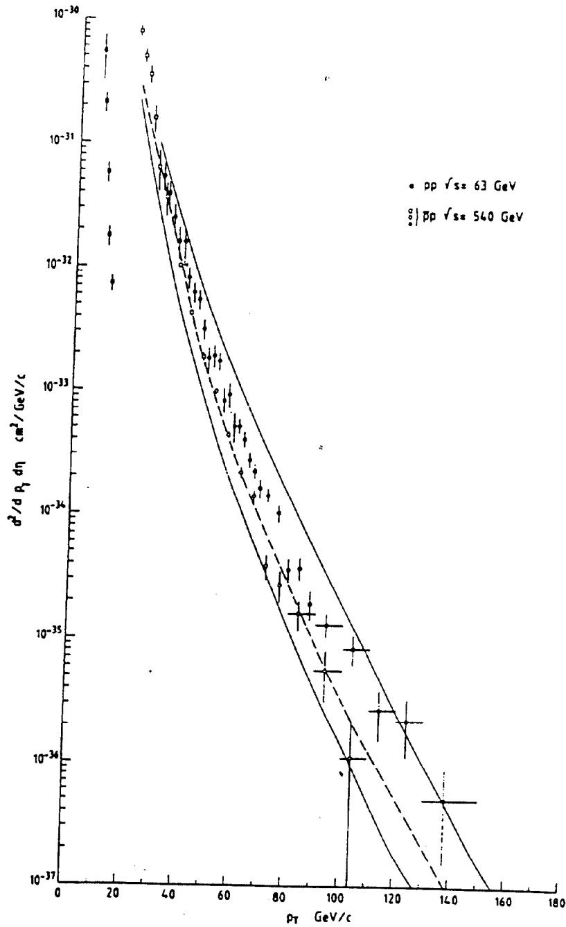
Figure 43: The jet cross section measured at the ISR and the CERN SPS by UA1 at rapidity = 0 . The dashed curve represents the original prediction as given in Horgan and Jacob 1981 and the solid curves indicate the range of predictions
