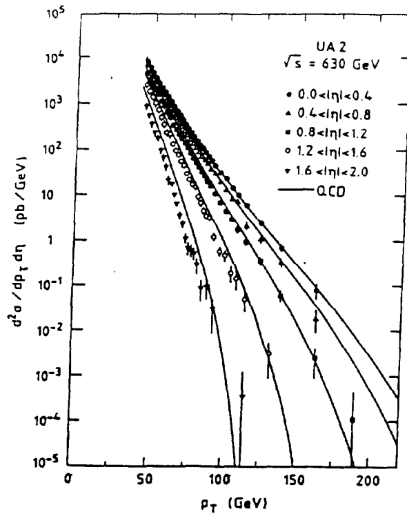
Figure 44: The inclusive jet cross section measured by the UA2 experiment for different pseudorapidities. The systematic error of 32% is not shown. The curves represent a LO QCD calculation with scale of E_t/2 , using the EHLQ parton distributions
