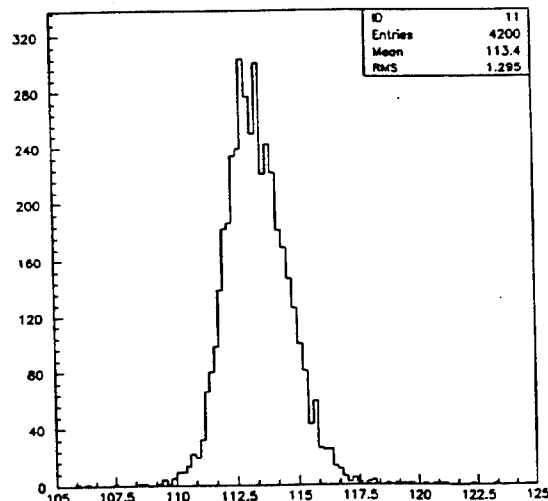
Figure 3, \frac{\Delta T}{T} = 3.414 \times 10^{-4} \times \# degrees at 201MHz, horizontal axis is in 201MHz degrees.
