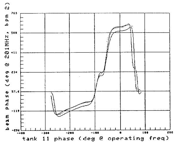
Figure 1. Upper curve is fit to data points. Lower curve is the target curve for Module 1.
