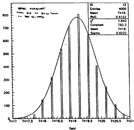
Figure 4. Regulation of spectrometer magnetic field.
