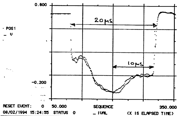
Figure 5. Beam position variation within a 20\mu\text{sec} macropulse.
