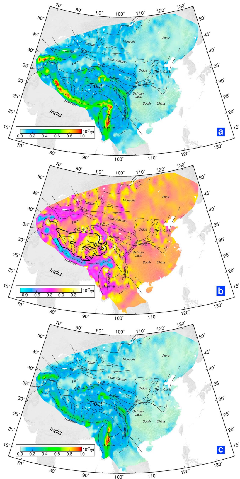
Figure 5. (a) Distribution of second invariant of strain rate tensor. (b) Dilatational strain rate field. Crustal extension is positive. Topography is Gaussian filtered with a 1^\circ width, and the 4750 m contour is shown by a black line. (c) Maximum shear strain rate field.
