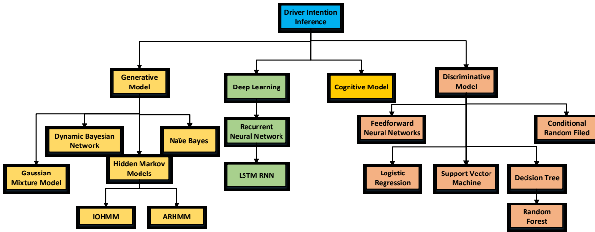
Fig. 5. Taxonomy of intention inference algorithms
