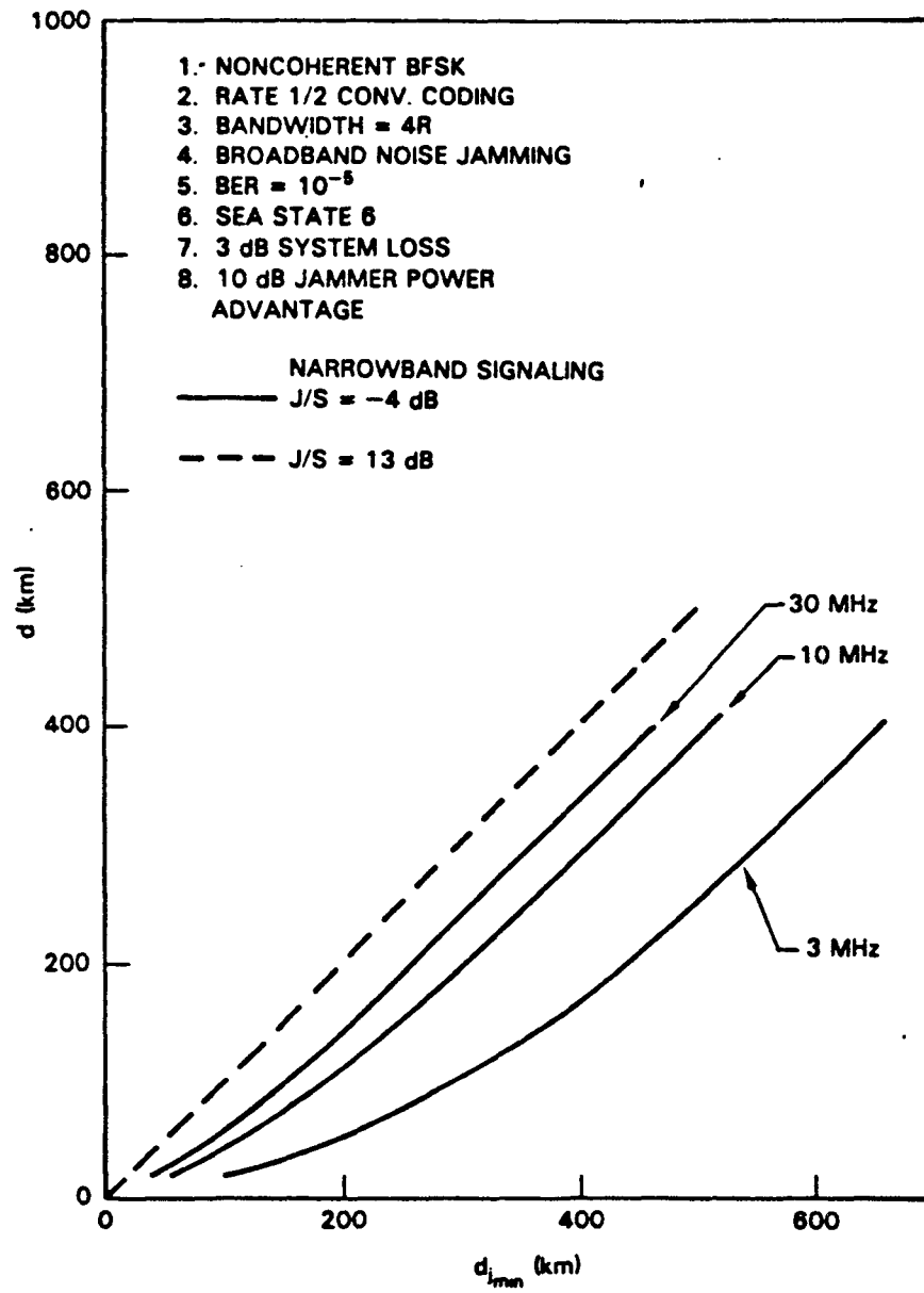
Fig. 8 - d_{jmin}(d) vs d for HF groundwave model and narrowband signaling
