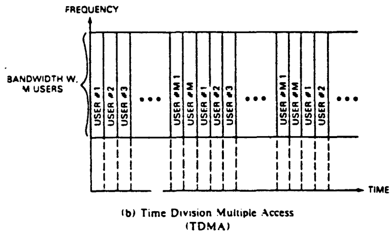
Fig. 4 — Fixed allocation multiple access methods
