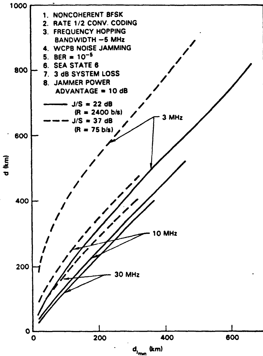
Fig. 7 - d_{jmin}(d) vs d for HF groundwave model and wideband signaling
