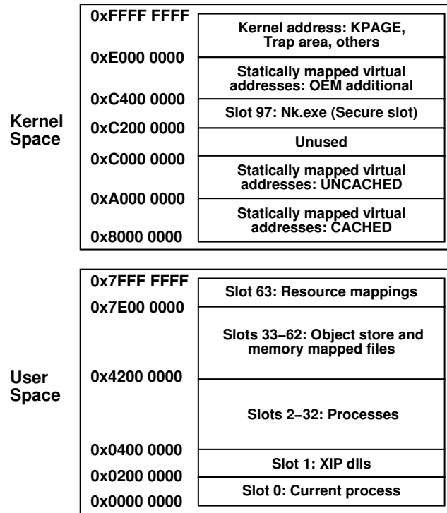
Figure 1. Virtual address space managed by WinCE.
