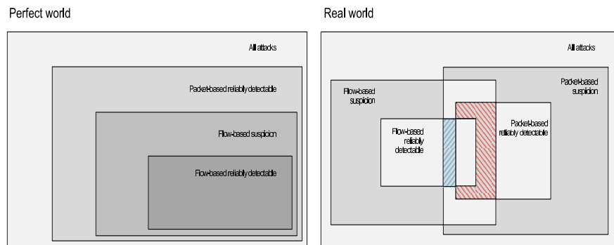
Figure 1 Detection Coverage [3]
