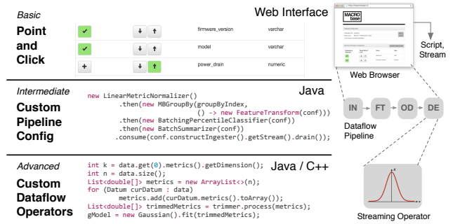
Figure 4: MacroBase Interfaces. MacroBase provides a range of interfaces for users of varying skill to perform analyses. A web-based point-and-click UI allows easy data exploration and export to command-line scripting and/or streaming. MacroBase also provides interfaces for users to configure custom pipelines of analytic operators (e.g., using feature transforms, or combining with relational operators including group-by) and for expert users to author their own streaming operators.
