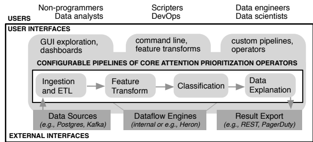
Figure 2: MacroBase System Architecture. MacroBase executes configurable dataflow pipelines of statistical analysis operators designed to prioritize attention in fast data streams.
