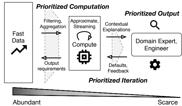
Figure 1: Fast Data System Design. A funnel of increasing scarcity from data to computational resources and humans guides the design of the system. Techniques for prioritizing computation and human attention exploit the resource imbalances at each level.
