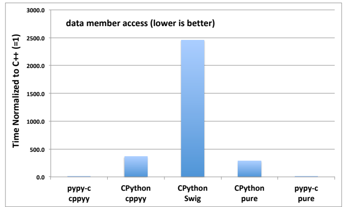
Fig. 4: Relative performance (compared to C++) of data member access in pypy-c . CPython using cpyyy , SWIG, and pure Python are shown for reference.
