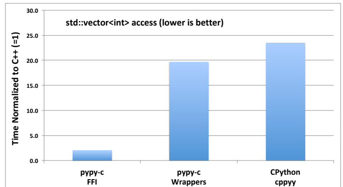
Fig. 5: Relative performance (compared to C++) of looping over an STL vector in pypy-c and CPython using cpyyy . SWIG not shown: it is \sim 350x slower.
