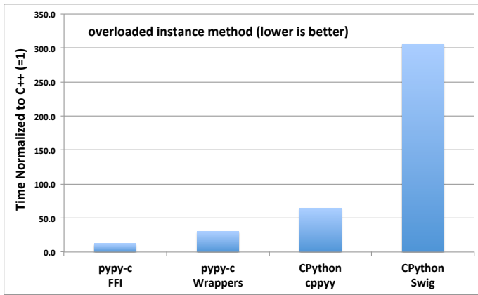
Fig. 3: Relative performance (compared to C++) of the FFI and wrapped paths for overloaded instance method calls. CPython using cpyyy and SWIG are shown for reference.
