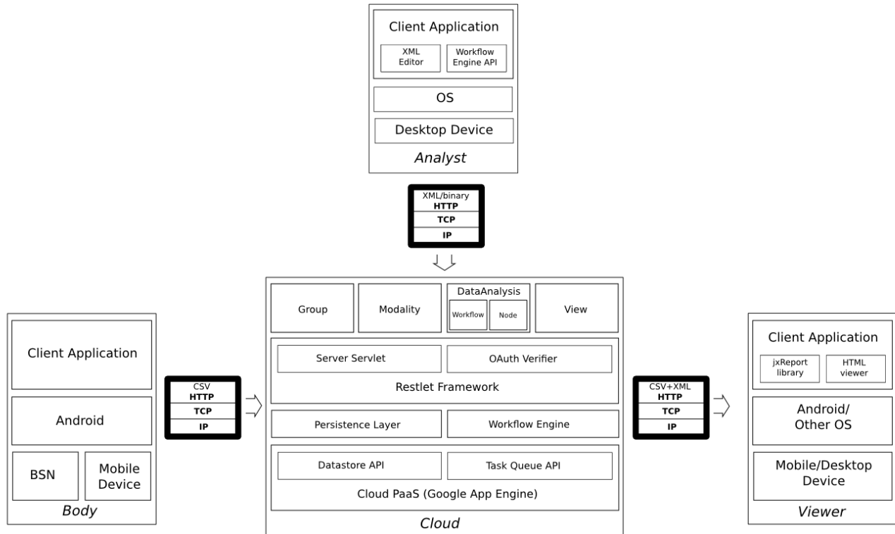
Figure 3. BodyCloud architecture.
