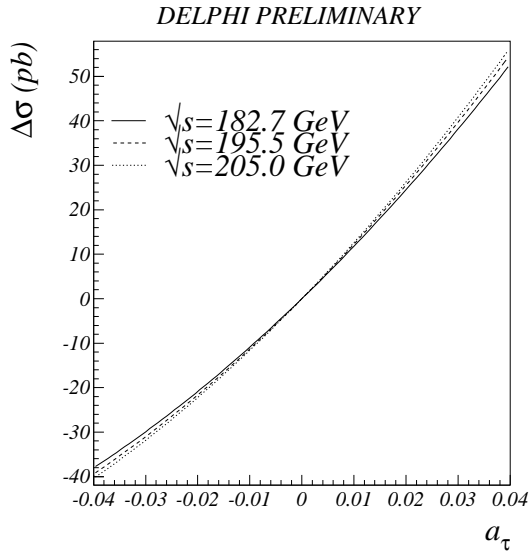
Figure 7: Total cross-section change as a function of anomalous magnetic moment and as a function of electric dipole moment.
