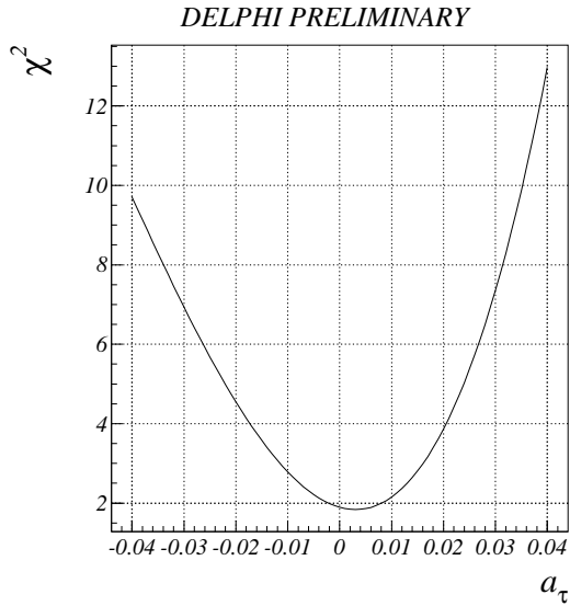
Figure 8: \chi^2 as a function of anomalous magnetic moment and as a function of electric dipole moment
