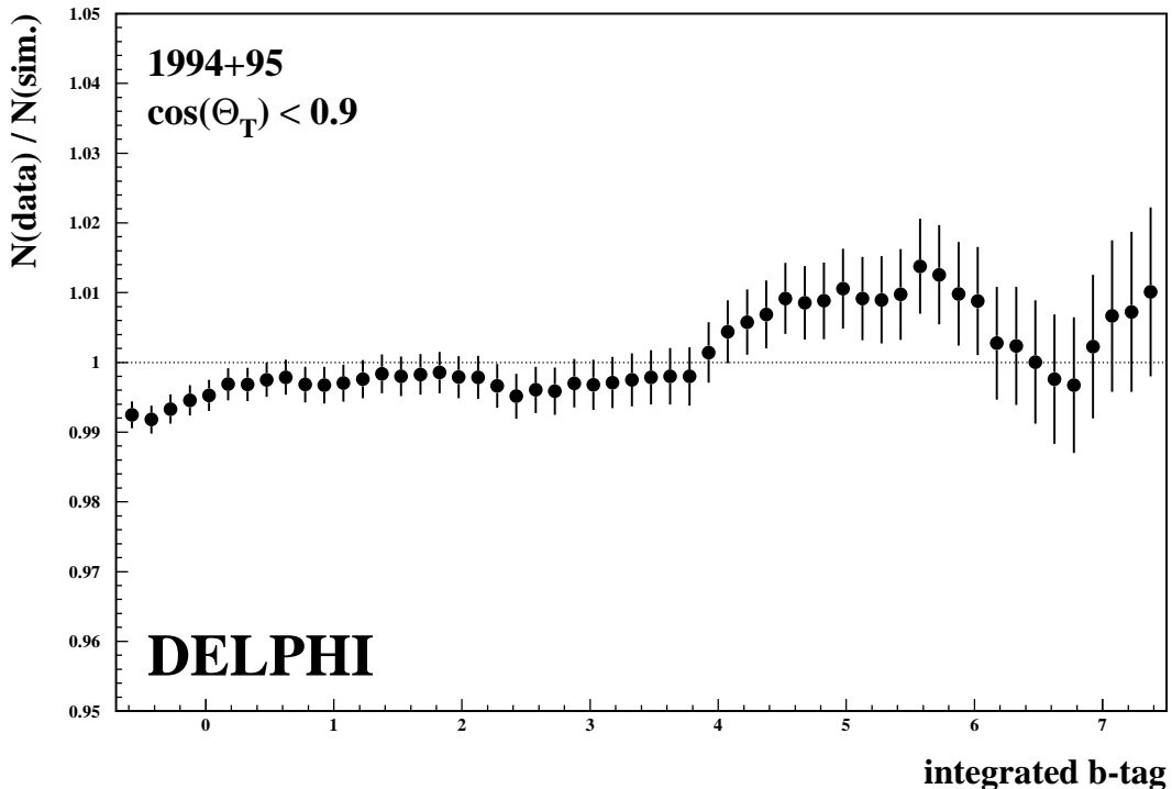
Figure 4: The ( integrated ) b\text{-tag} ratio of real to simulated events after application of the correction functions to simulated b and c quark events. The data are from the 1994+95 DELPHI data set. Different correction functions for the \cos\theta_{\vec{\tau}} intervals of [0.0, 0.5] , [0.5, 0.7] and \geq 0.7 were applied before integrating over the full polar angle.
