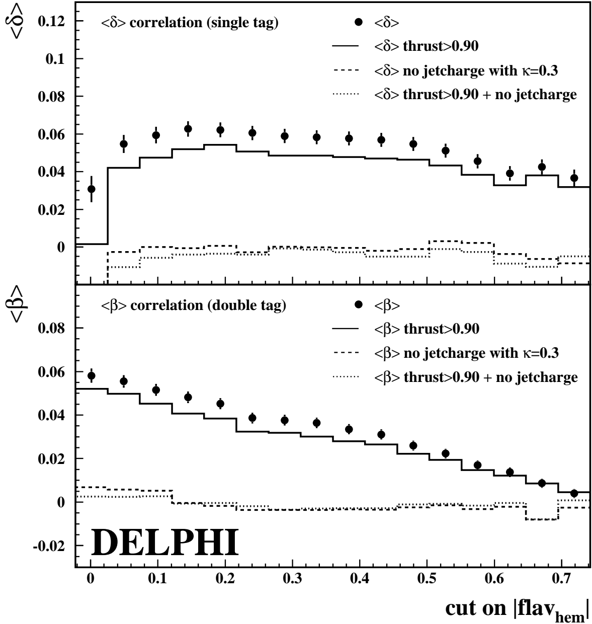
Figure 10: The mean of the correlations \delta and \beta of 1994 simulation as a function of the cut on the charge tag output |flav_{hem}| . Besides the full hemisphere charge network (points) results using modified networks without the jet charge input for \kappa = 0.3 and both with an additional cut on the thrust value, |\vec{T}| > 0.9 , are shown. The statistical uncertainties on the quantities represented by lines are not drawn, but they are slightly larger than those shown for the points.
