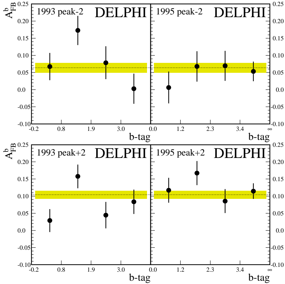
Figure 16: The A_{FB}^b results for the 1993 and 1995 off-peak runs and each interval in b -tag with their statistical errors. The lines in the upper and lower plots are the results of \chi^2 -fits that were run separately at \sqrt{s} = 89.449 and 92.990 GeV. The band shows again the statistical uncertainty.
