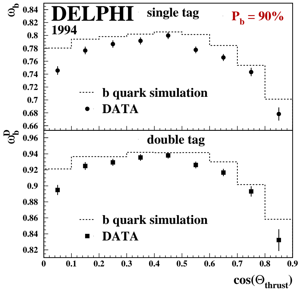
Figure 8: The probability to identify b quarks correctly for data and simulation for the year 1994. The upper plot shows the result for single tagged events, the lower for double tagged events. See text for details.
