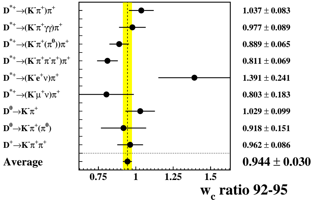
Figure 12: The ratio of real data to simulation in the c quark charge identification w_c provided by a flav_{\text{hem}} tag in a hemisphere opposite a reconstructed D . The final result is decomposed into the 9 different decay channels used in [16].
