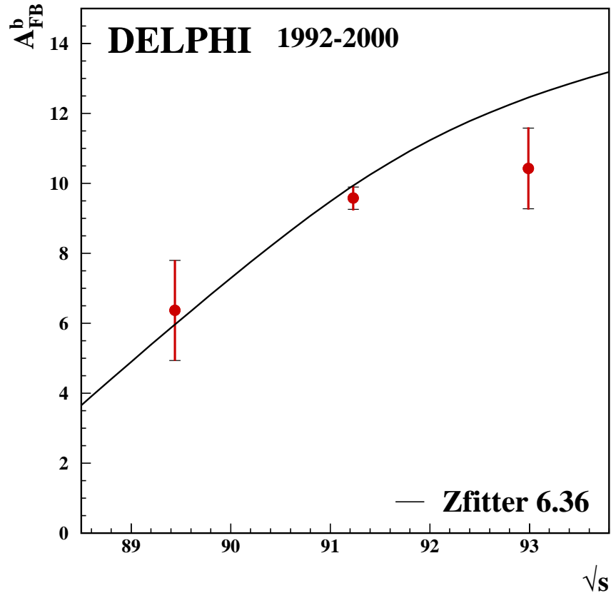
Figure 23: The A_{FB}^b results versus the centre-of-mass energy. The total errors (bars) are only slightly larger than the statistical (flags). The curve represents the Standard Model prediction obtained from ZFITTER [15].
