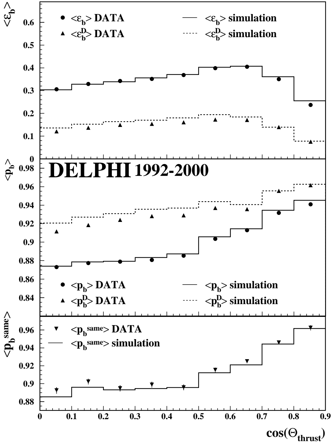
Figure 7: The b efficiencies \epsilon_b and \epsilon_b^D and the purities p_b and p_b^D for single and double unlike-sign tagged events as a function of the polar angle. The purity p_b^{same} for double like-sign tagged events is relevant for measuring the charge tagging probability, w_b^{(D)} .
