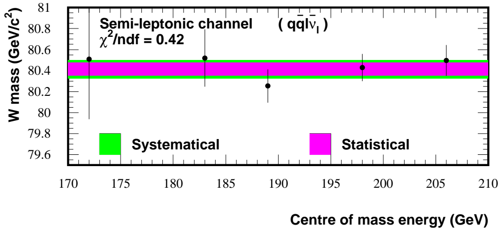
Figure 4: Fitted W mass as function of the centre-of-mass energy in the (a) q\bar{q}'\bar{q}q' and (b) \ell\bar{\nu}_\ell q\bar{q}' analysis channels are shown. The statistical and systematic components of the combined W mass uncertainty are shown, where the shaded areas are proportional to the ratio of the squares of the two component errors.
