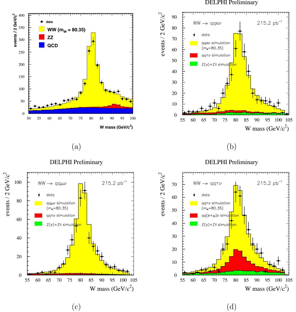
Figure 3: The distribution of the reconstructed W masses in the 2000 data from a kinematic fit with five constraints imposed in the (a) q\bar{q}'q\bar{q}' , (b) e\bar{\nu}_e q\bar{q}' , (c) \mu\bar{\nu}_\mu q\bar{q}' and (d) \tau\bar{\nu}_\tau q\bar{q}' analysis channels. In the q\bar{q}'q\bar{q}' channel, only the jet pairing with the highest probability is included in this figure.
