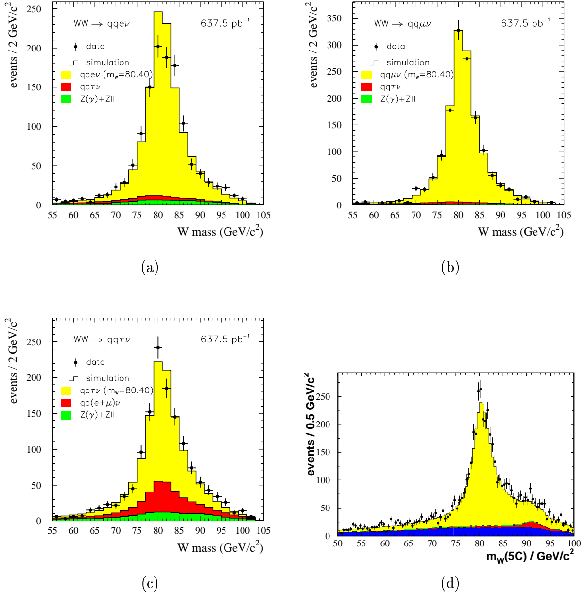
Figure 8: The distribution of the reconstructed W masses from a kinematic fit with five constraints imposed in the (a) e\bar{\nu}_e q\bar{q}' , (b) \mu\bar{\nu}_\mu q\bar{q}' , (c) \tau\bar{\nu}_\tau q\bar{q}' and (d) q\bar{q}'\bar{q}q' analysis channels. In the q\bar{q}'\bar{q}q' channel, only the jet pairing with the highest probability is included in this figure. Figure (d) will be changed to the same style as (a),(b),(c) for Draft 2
