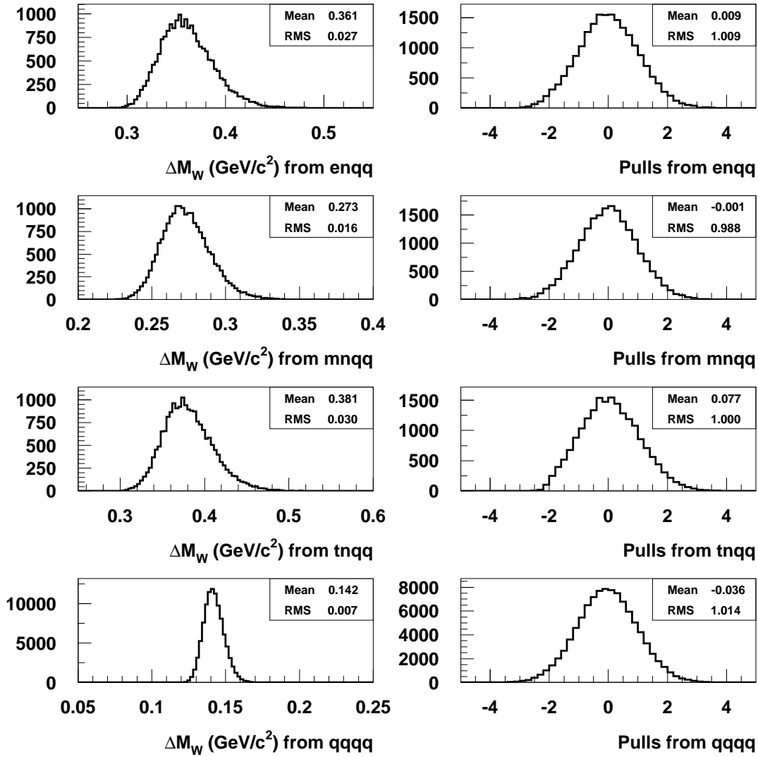
Figure 10: The errors (left) and pulls (right) of the W mass fits for each semi-leptonic analysis channel and the fully-hadronic channel. These plots were obtained using simulated event samples with the same statistics as the data sample collected at 200 GeV. The errors obtained on the fits to the data samples were 365 \text{ MeV}/c^2 for the e\bar{\nu}_e q\bar{q}' analysis, 282 \text{ MeV}/c^2 for \mu\bar{\nu}_\mu q\bar{q}' , 438 \text{ MeV}/c^2 for \tau\bar{\nu}_\tau q\bar{q}' and 149 \text{ MeV}/c^2 for q\bar{q}'\bar{q}q' .
