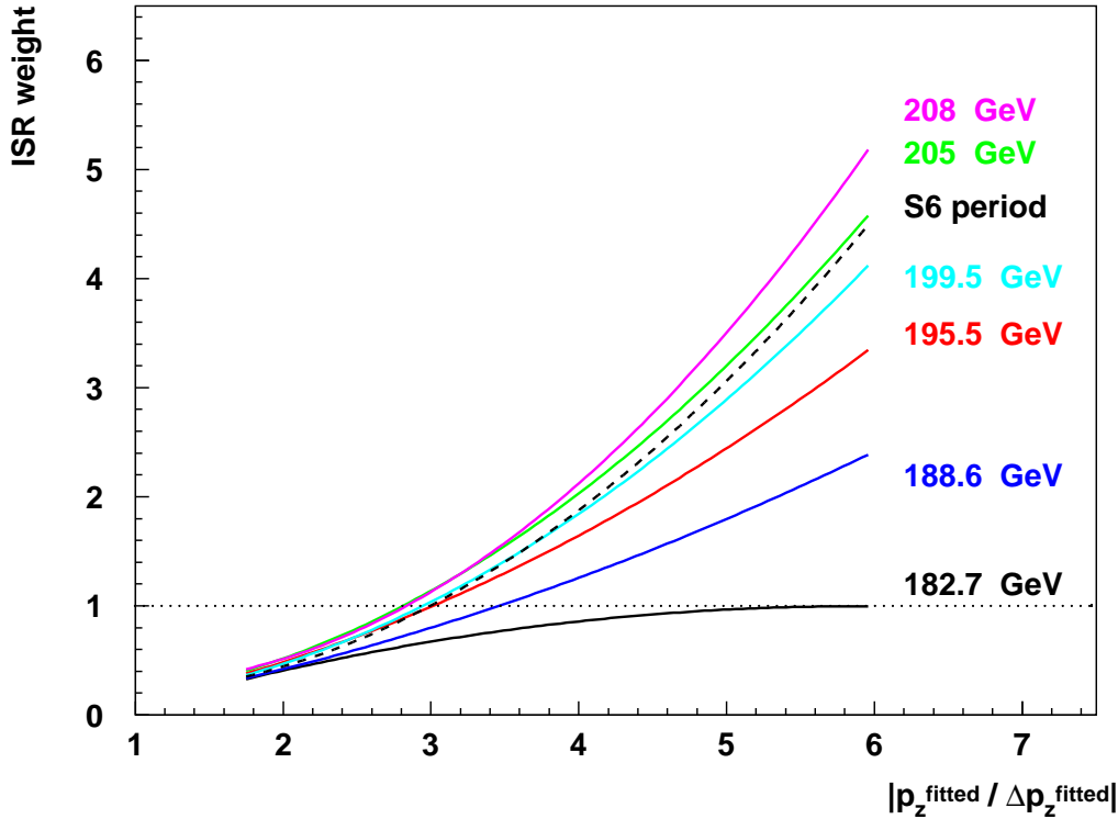
Figure 7: Parameterised weight given to the ISR solution of the kinematic fit as a function of the |p_z^{\text{fitted}}|/\sigma_{p_z} value of the event for different centre-of-mass energies. The period with a damaged TPC sector (S6) is indicated with a dashed line.
