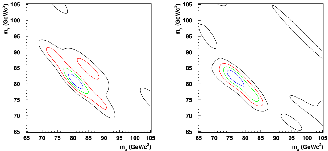
Figure 6: Examples of a reconstruction hypothesis weighted sum of two-dimensional probability ideograms (see text) for a four-jet (left) and five-jet (right) hadronic event. The ideograms include terms from each potential jet-pairing, three jet clustering algorithms and possible ISR emission. The first four sigma contours are shown.
