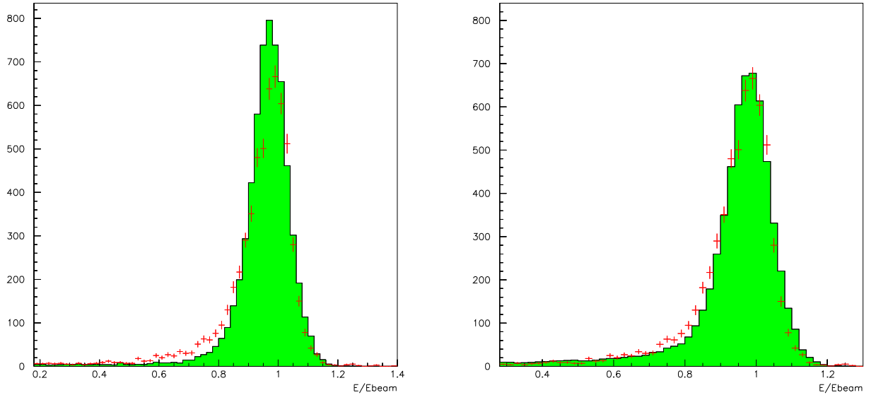
Figure 11: The ratio E/E_{\text{beam}} for electrons in the endcaps from Bhabha events recorded at the Z peak in 1998. The histogram is the simulation and the points are the data. The left plot is the raw distribution, while the right one is after the bremsstrahlung correction discussed in the text. The resolution correction (see text) has also been applied.
