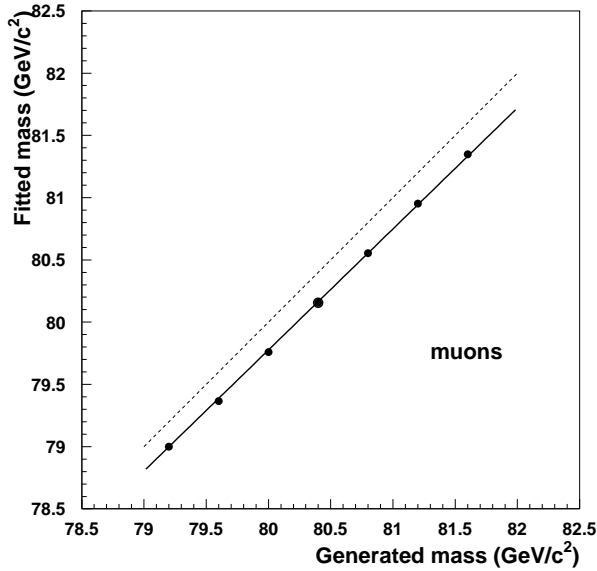
Figure 9: W mass calibration curve in the \mu\bar{\nu}_\mu q\bar{q}' channel at \sqrt{s} = 189 \text{ GeV} . The dashed line indicates the result that would be obtained without any analysis bias.
