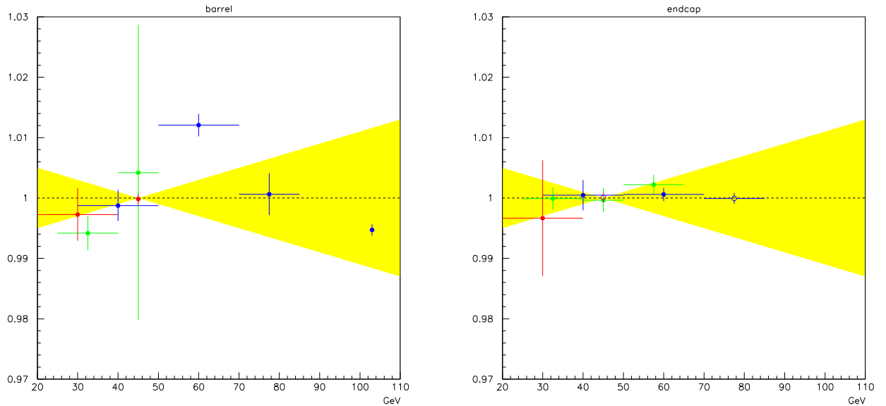
Figure 12: The double ratio of reconstructed and true average energy values in data and simulation \langle E_{rec}/E_{true} \rangle_{data}/\langle E_{rec}/E_{true} \rangle_{MC} for data taken in 2000. The shaded area represents the quoted systematics due to a possible dependence of the energy calibration with the electron energy. The left hand plot is for electrons observed in the barrel electromagnetic calorimeter and the right hand plot for electrons in the endcap. Note that, by construction, the Bhabha point at 45 GeV is at one.
