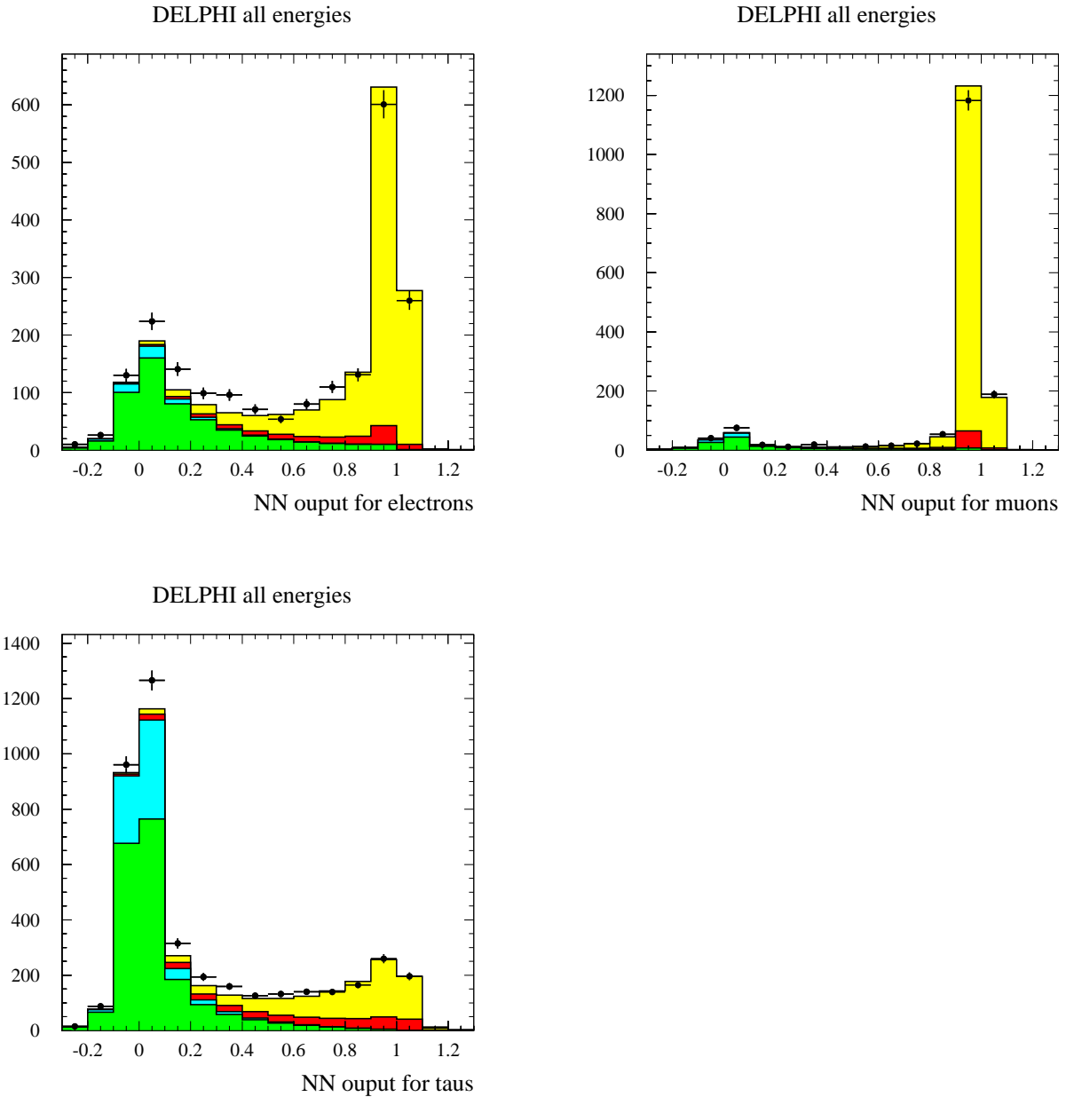
Figure 2: The output of the neural network used for the selection of the semi-leptonic channels for the data sample recorded at \sqrt{s} = 183 - 209 GeV. The data are indicated by the data points with error bars. The W^+W^- simulation events where the correct lepton identification has been made are shown in yellow, the events in red are other semi-leptonic W^+W^- events, fully-hadronic W^+W^- decay events are in blue, with the green area indicating the background events.
