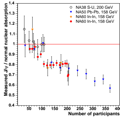
Figure 5. J/\psi suppression pattern measured in S+U, In+In and Pb+Pb, as a function of N_{\text{part}} .
