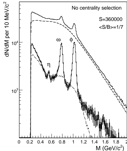
Figure 1. Mass distribution of opposite-sign dimuons (upper histogram), combinatorial background (dashed), signal fake matches (dashed-dotted), and resulting signal (lower histogram with error bars).
