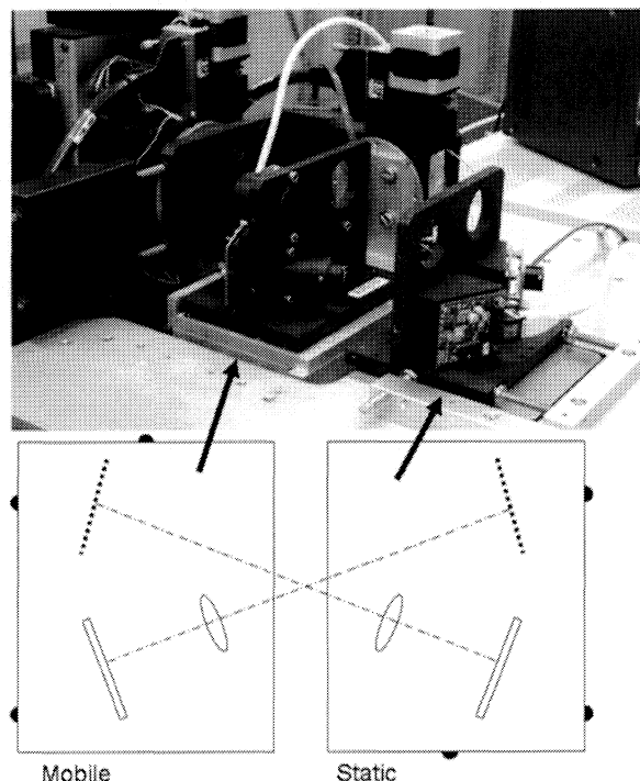
Figure 4: picture and top view drawing of the praxial sensor (top and bottom respectively).
