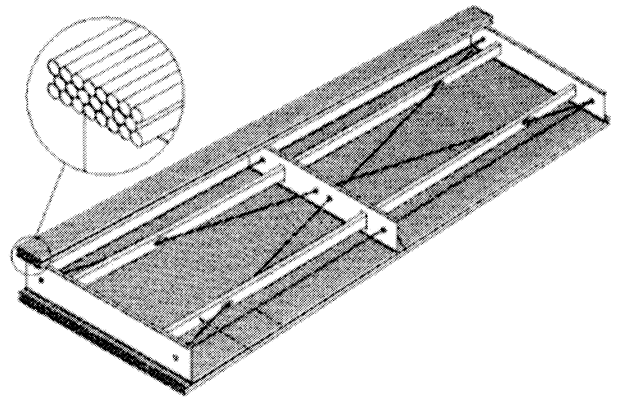
Figure 2: A muon chamber.
