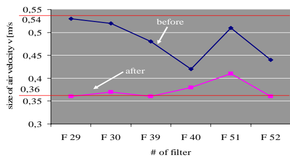
Figure 2: air velocity distribution measured on filter units before / after re adjustment of air distribution flaps
