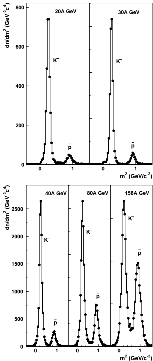
FIG. 1: Mass squared histograms for TOF-identified kaons and antiprotons in Pb+Pb reactions at 20, 30, 40, 80 and 158 A GeV beam energies. dE/dx cuts have been applied to the data to reject most of the pions. The particle momenta range from 3 to 10 GeV/ c .
