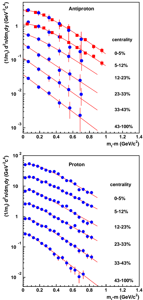
FIG. 2: (Color online) Transverse mass distributions for antiprotons and protons [19] in the rapidity interval 2.4 < y < 2.8 for the six centrality classes in 158A GeV Pb+Pb collisions. The circle and square points denote the data obtained with the trigger settings selecting minimum bias and central collisions, respectively. The errors are statistical. The curves through the measured points represent the two-exponential fit of Eq. (1) to the data. For clarity, the spectra are scaled down by a factor of 2 successively from the uppermost data.
