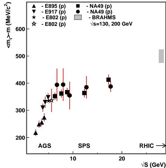
FIG. 5: (Color online) The mean transverse mass \langle m_t \rangle - m for \bar{p} and p at midrapidity as a function of the center-of-mass energy per nucleon pair \sqrt{s_{NN}} in central Pb+Pb collisions at SPS energies (NA49) together with data for central Au+Au collisions from the AGS [33, 34, 35] and RHIC [36]. The errors are statistical.
