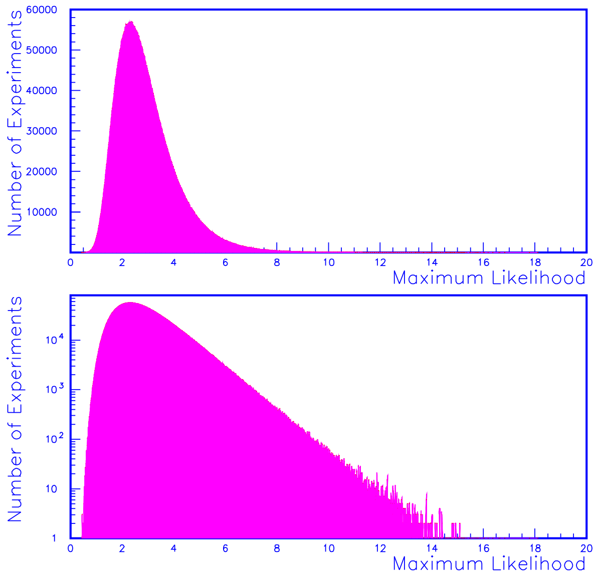
Figure 3: The Maximum Likelihood output for 13,450,000 background-only MC experiments. The top plot is in linear scale while the bottom plot is in log scale.
