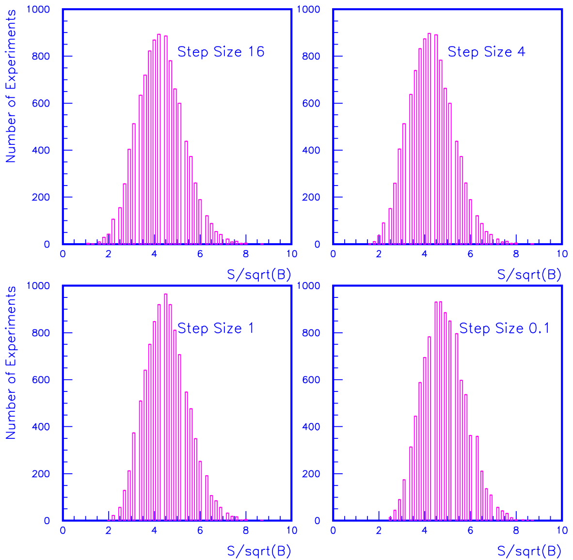
Figure 4: The maximum S/\sqrt{B} from “Sliding-Window” approaches with step sizes of 16, 4, 1, and 0.1 for the best-case scenario 10,000 MC experiments each with 20 signal events embedded.
