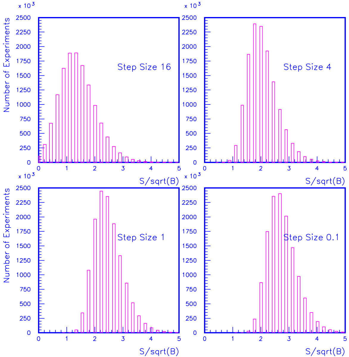
Figure 2: The maximum S/\sqrt{B} from “Sliding-Window” approaches with step sizes of 16, 4, 1, and 0.1 for the 13,450,000 background-only MC experiments.
