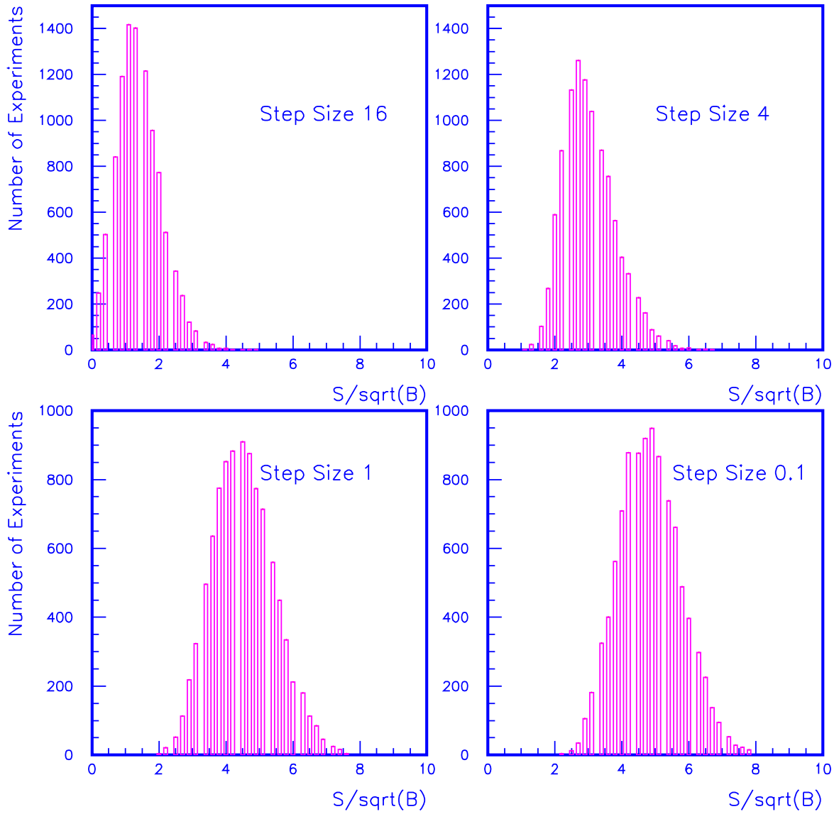
Figure 5: The maximum S/\sqrt{B} from “Sliding-Window” approaches with step sizes of 16, 4, 1, and 0.1 for the worst-case scenario 10,000 MC experiments each with 20 signal events embedded.
