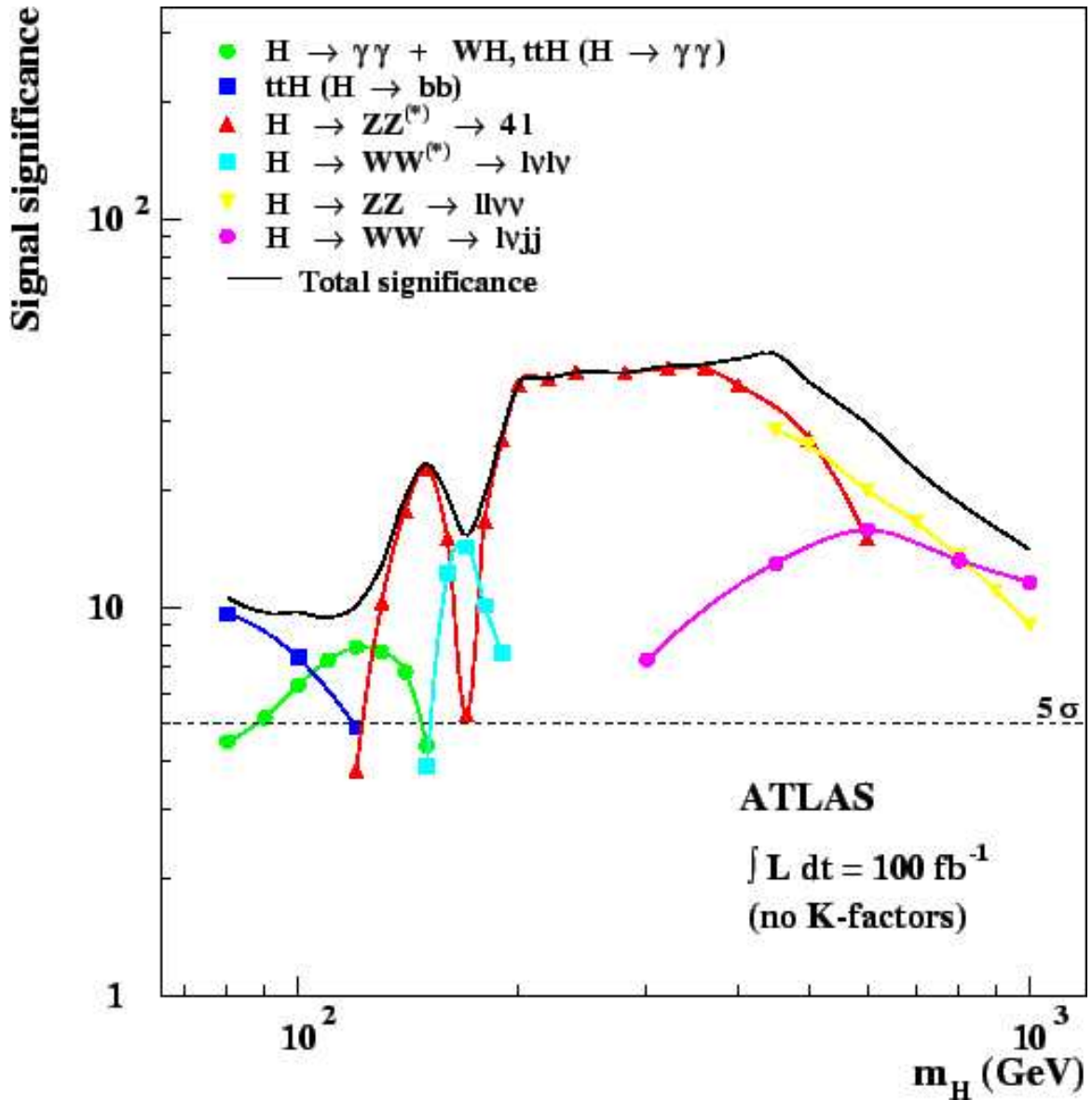
Figure 1: The expected significance for observing SM Higgs boson as a function of the Higgs mass at ATLAS. The statistical significances are plotted for individual channels, as well as for the combination of all channels, assuming an integrated luminosity of 100 \text{ fb}^{-1} . Each point in the curve is calculated based on the S and B values of a narrow mass window using the “Sliding-Window” method.
