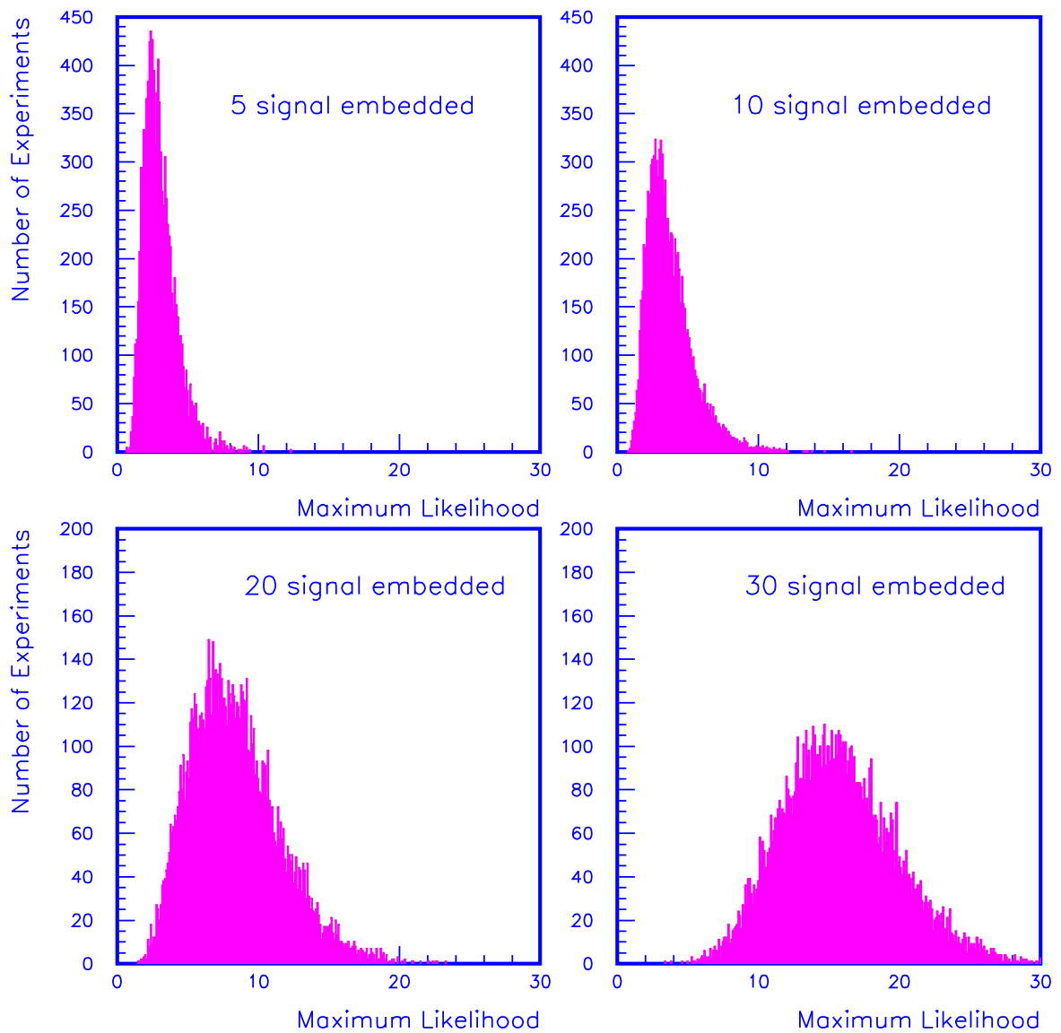
Figure 6: The Maximum Likelihood output for MC experiments with 5, 10, 20, 30 signal events embedded respectively.
