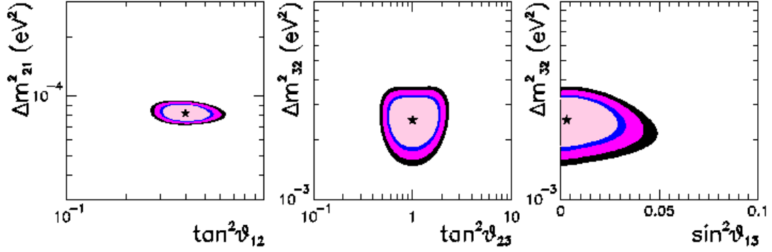
Figure 1: Current experimental constraints on the three mixing angles \theta_{12} , \theta_{23} , and \theta_{13} and their dependence on the two known mass-squared differences m_{12}^2 and m_{23}^2 . The star indicates the most likely solution. Figure taken from [1].
