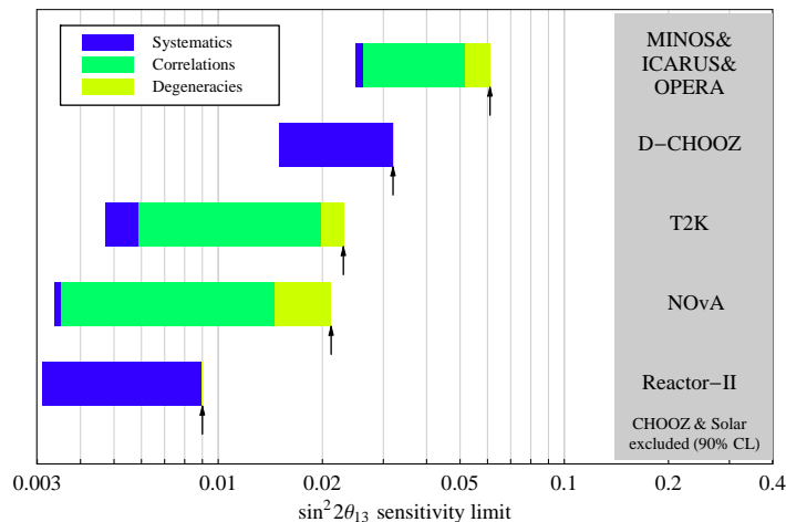
Figure 3: The \sin^2 2\theta_{13} sensitivity limit at the 90% CL for MINOS, ICARUS, and OPERA combined, Double-Chooz, T2K, 2 nd generation reactor experiment (Reactor-II), and NOvA. The left edges of the bars are obtained for the statistics limits only, whereas the right edges are obtained after successively switching on systematics, correlations, and degeneracies, i.e., they correspond to the final \sin^2 2\theta_{13} sensitivity limits. The gray-shaded region corresponds to the current \sin^2 2\theta_{13} bound at 90% CL. For the true values of the oscillation parameters, we use |m_{31}^2| = 2.0 \cdot 10^3 \text{ eV}^2 , \sin^2 2\theta_{23} = 1 , m_{21}^2 = 7.0 \cdot 10^5 \text{ eV}^2 , \sin^2 2\theta_{12} = 0.8 [14,67{69}], and a normal mass hierarchy. Figure extended version from Ref. [66].
