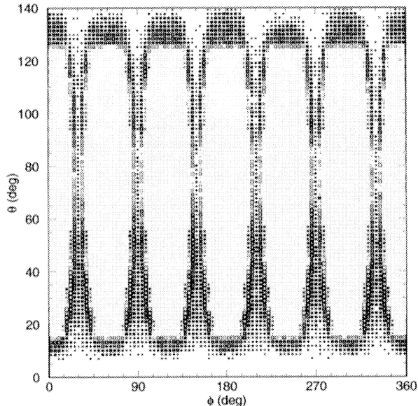
FIG. 4: Angular coverage for the identified protons. The light gray areas represent the fiducial regions of the six CLAS sectors inside which the protons for the present analysis have been accepted.
