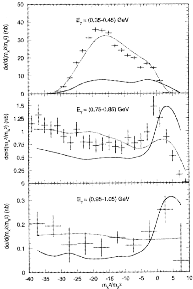
FIG. 23: Distributions of m_X^2/m_*^2 (see Eq. (11)) for the star configuration exemplified by three 0.1-GeV-wide photon-energy bins. The dotted lines represent the phase-space predictions, multiplied by the constants used to normalize the full-Dalitz cross sections, while the solid curves are the full-model results.
