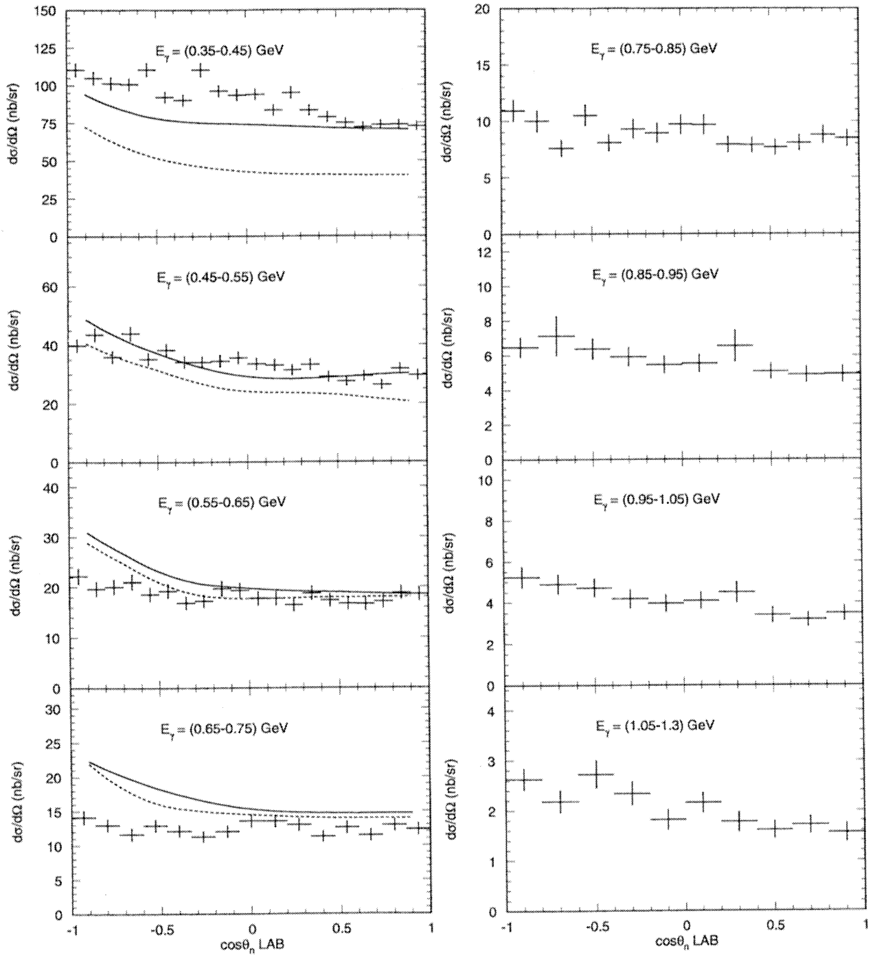
FIG. 16: Differential cross sections integrated over the CLAS for the neutron-spectator kinematics with respect to \cos \theta of the neutron in the laboratory frame for photon energies between 0.35 and 1.30 GeV. The data are compared with the results of the full model (solid curves) and those of the one- plus two-body-only model (dashed curves), for 0.35 < E_\gamma < 0.75 GeV only, because at higher energies the model calculations differ by more than an order of magnitude from the data.
