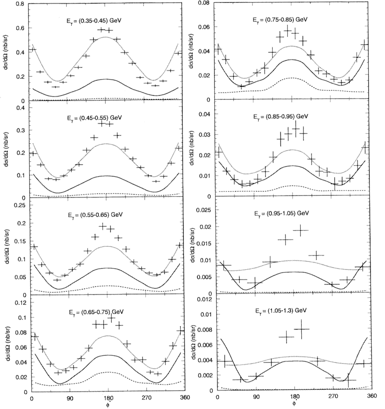
FIG. 22: CLAS-integrated differential cross sections with respect to \phi^* for the star configuration. The data, for photon energies between 0.35 GeV and 1.30 GeV, are compared with the full-model results (solid curves) and the one- plus two-body-only part (dashed curves). The dotted curves are the phase-space distributions, multiplied, for each photon-energy bin, by the constants used to normalize the full-Dalitz cross sections.
