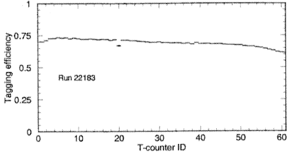
FIG. 9: Tagging efficiency as a function of T-counter number measured in one particular low-flux run. The average efficiency is about 70%.
