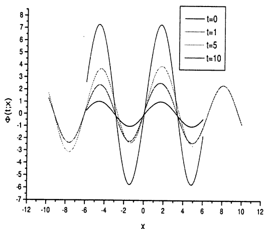
Figure 1: \Phi -plots for periodic initial conditions
