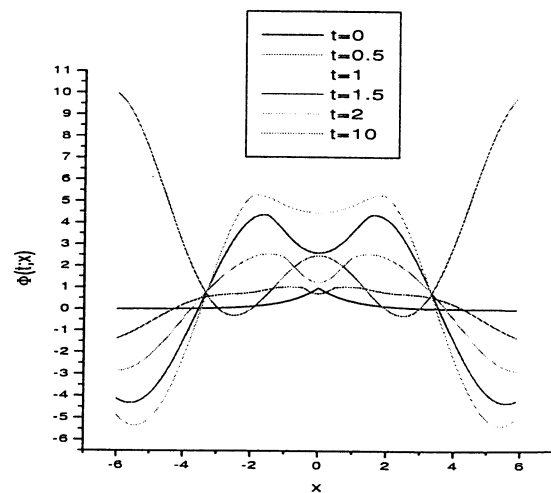
Figure 2: \Phi -plots for exponentially decreasing initial conditions
