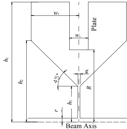
Fig. 5 2-D profile of the couple cell
