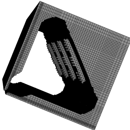
Fig. 1 3-D MAFIA picture of one quadrant of one section without end cells
