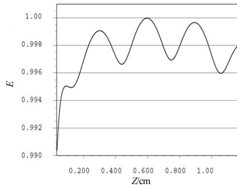
Fig. 4 The distribution of the transverse electrical fields along the longitudinal axis
