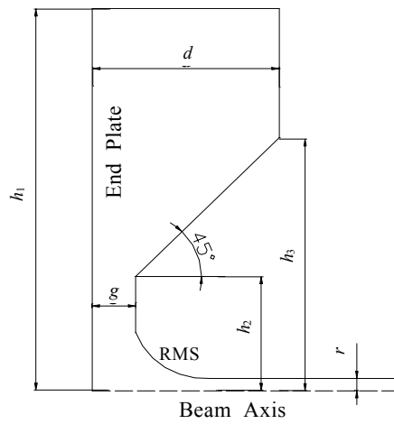
Fig. 3 2-D profile of the beginning cell
