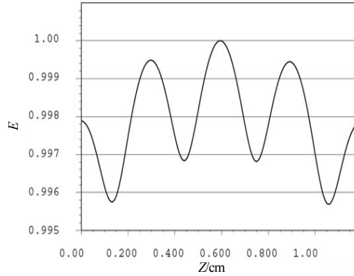
Fig. 2 The distribution of the electrical fields along the transverse longitudinal axis
