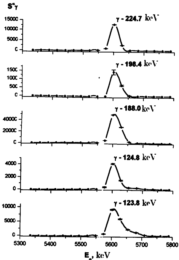
Fig. 1 Intensity of (\alpha\text{-}\gamma) -coincidences of \gamma -rays from the 224.6-keV level as a function of the \alpha -particle energy in the window. The distributions for \gamma -123.8 and \gamma -124.8 keV are broadened on the large E_\alpha side because of summation of pulses from \alpha -particle and pulses from ICE of transitions from the 100.9 and 99.8-keV levels
