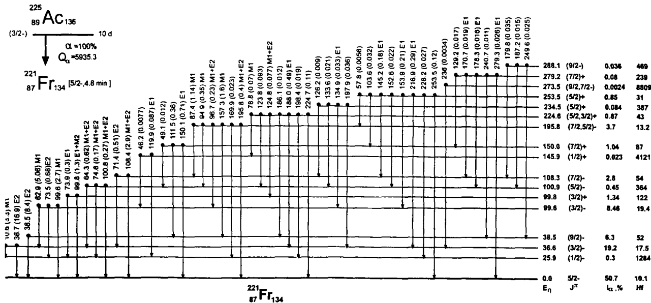
Fig. 4 225 Ac decay scheme. Solid lines represent \gamma -transitions whose position is proved by the ( \alpha - \gamma )-coincidences, dashed lines represent \gamma -transitions whose position is not in conflict with the ( \alpha - \gamma )-coincidences. Shown above the transitions are their energies, total (including conversion) intensities (in parentheses), and experimental multipolarity data. Near the level energies there are spins, parities, intensities of the \alpha -decay to the levels, and hindrance factors.
