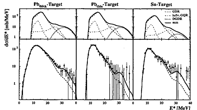
FIG. 7: (Color online) Lower panels: Experimental excitation energy spectra for ^{136}\text{Xe} (700 MeV/nucleon) on the three targets. The solid lines show the result of the data analysis including cross sections for GDR, GQR, and DGDR excitations, the dashed lines those without DGDR excitations. The calculated spectra are convoluted with the response of the detector system. Upper panels: Calculated spectra prior to convolution for the GDR, isovector and isoscalar GQR, the DGDR, and their sum, as indicated in figure.
