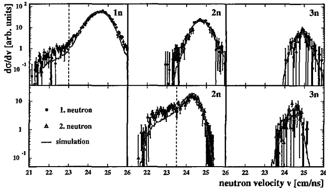
FIG. 6: (Color online) Neutron velocity spectra in the laboratory frame measured with the thick Pb target. Left-hand panel: for the one-neutron decay channel. Middle panels: for the first and second neutron detected for the two-neutron decay channel. Right-hand panels: for the first and second neutron detected for the three-neutron decay channel. The solid curves show the result from the Monte-Carlo simulation. The dashed line indicates the cut on slow neutrons, see text.
