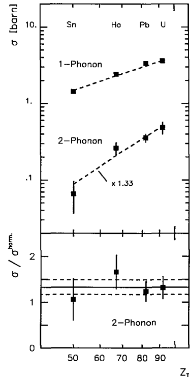
FIG. 9: Upper panel: Integrated cross sections for the GDR and the DGDR in ^{208}\text{Pb} measured on different targets of nuclear charge Z_T . The dashed lines interpolates cross-section predictions from the semi-classical calculation; in case of the DGDR, the calculated values are multiplied by a factor of 1.33. (Lower panel). Ratio of the experimental cross sections for the DGDR in ^{208}\text{Pb} to the ones calculated in the harmonic limit. The mean value and its error are indicated by solid and dashed lines, respectively.
