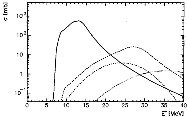
FIG. 15: Cross section distributions for the GDR (solid line) and double-phonon states populated in ^{208}\text{Pb} projectiles (640 MeV/nucleon) impinging on a Pb target: DGDR (dashed line); \text{GDR} \otimes \text{GQR}_{is} (dashed-dotted line); \text{GDR} \otimes \text{GQR}_{iv} (dotted line).
