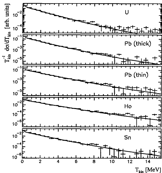
FIG. 10: Neutron kinetic energy spectra, 1/T_{kin}d\sigma/dT_{kin} , in the ^{208}\text{Pb} projectile center-of-mass frame for different targets as indicated and for events with emission of one neutron. Solid lines represent Maxwell distributions with adjusted slope parameter T_0 , see eq.( 4), after folding with the experimental response.
