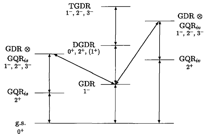
FIG. 14: Excitation pathways adopted for the coupled-channels calculation estimating cross sections for two-phonon states of type GDR \otimes GQR. TGDR denotes three-phonon giant dipole resonances.
