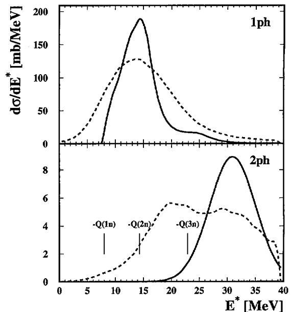
FIG. 3: (Color online) Upper panel: The solid line shows the energy-differential electromagnetic cross section of one-phonon giant dipole and quadrupole resonances excited in ^{136}\text{Xe} projectiles (700 MeV/nucleon) impinging on a thick Pb target as calculated within the semiclassical approach using resonance parameters from the literature (see Table I). The dashed line represents the modification of this distribution due to the experimental filter. Lower panel: same as upper panel, however for the double-phonon giant dipole resonance as obtained from the folding model. Thresholds (-Q) for the decay into 1, 2, and 3 neutrons are indicated.
