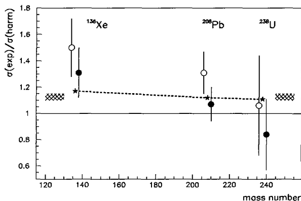
FIG. 16: Experimental DGDR cross sections relative to their harmonic values prior to (open circles) and after (filled circles) subtraction of contributions from two-phonon states of type \text{GDR} \otimes \text{GQR} for the three measured nuclei on a Pb target. The hatched areas indicate the expected increase of the cross sections due to phonon damping during the collision. Star symbols (connected by a dashed line) reflect the increase of cross section due to an anharmonic dipole response relative to the harmonic response (see text).
