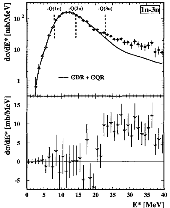
FIG. 5: (Color online) Upper panel: Experimental differential cross section d\sigma/dE^* for ^{136}\text{Xe} and the thick Pb target. Threshold energies ( -Q ) for the separation of one to three neutrons are indicated. The solid line represents the calculated sum of cross sections for one-phonon giant dipole and quadrupole resonances. Lower panel: Difference in measured and calculated cross sections from upper panel.
