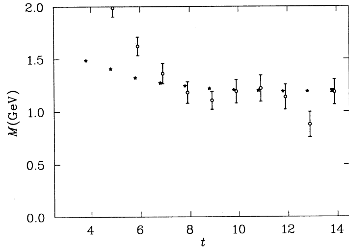
Figure 5. Effective mass plot for correlation functions of the standard \rho -meson interpolator \bar{q}^a \gamma_j q^a and the hybrid \rho interpolator \bar{q}^a \gamma_4 \gamma_5 B_j^{ab} q^b .
