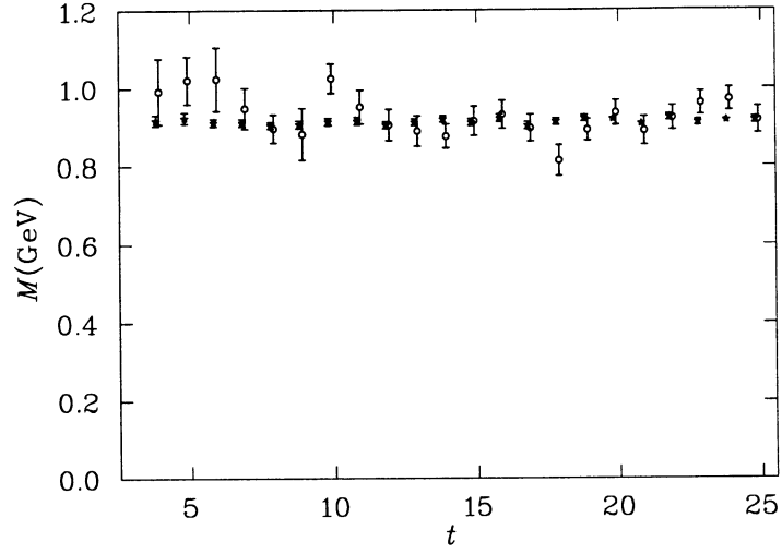
Figure 4. Effective mass plot for correlation functions of the standard axial-vector pion interpolator \bar{q}^a \gamma_5 \gamma_4 q^a and the hybrid pion interpolator \bar{q}^a \gamma_4 \gamma_j B_j^{ab} q^b .
