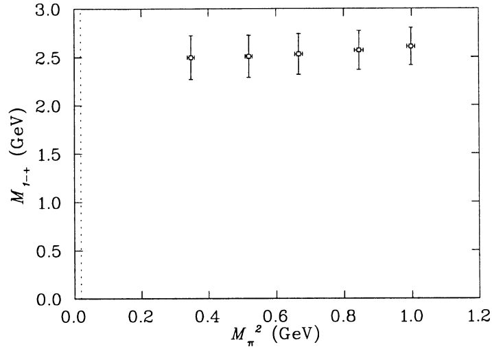
Figure 2. Effective mass plot of the 1^{-+} exotic meson obtained from the hybrid interpolating field \epsilon_{jkl}\bar{q}^a\gamma_k B_l^{ab}q^b , vs m_\pi^2 derived from the standard pion interpolator \bar{q}^a\gamma_5 q^a .
