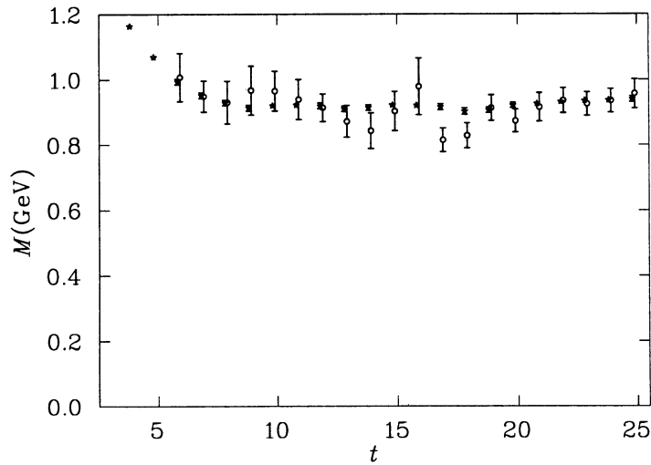
Figure 3. Effective mass plot for correlation functions of the standard pion interpolator \bar{q}^a\gamma_5 q^a and the hybrid pion interpolator \bar{q}^a\gamma_j B_j^{ab}q^b .
