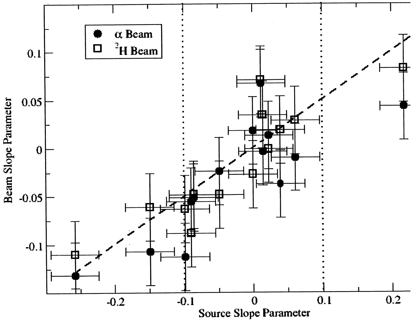
Fig. 6: Correlation between the slope parameters obtained via the alpha source test and those obtained via the 220 MeV alpha beam test (solid points) and the 110 MeV deuteron beam test (open points).
