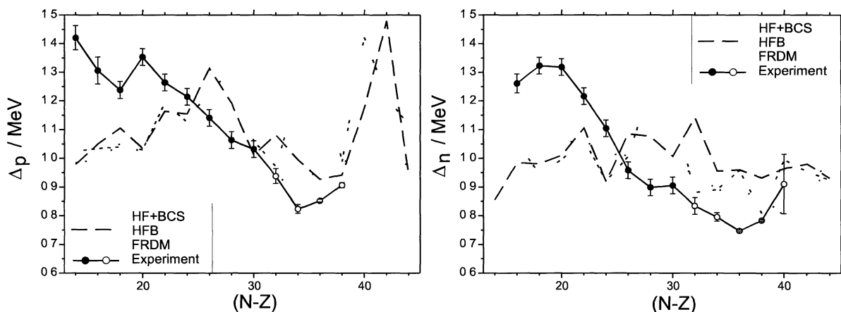
Figure 4 Measured isospin dependence of proton (left panel) and neutron (right panel) pairing-gap energies for even-even tungsten isotopes compared with nuclear models [10, 11]. The experimental values are taken from this work and Ref. [8]. The full circles represent our new values.
