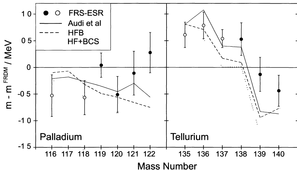
Figure 5 Preliminary experimental data of new masses for Te and Pd isotopes compared with the AME prediction [8] and with theories (HFB[10], HF+BCS[10], FRDM[11]). The isotopes which were measured for the first time are indicated by full circles. The open circles represent previously known masses.
