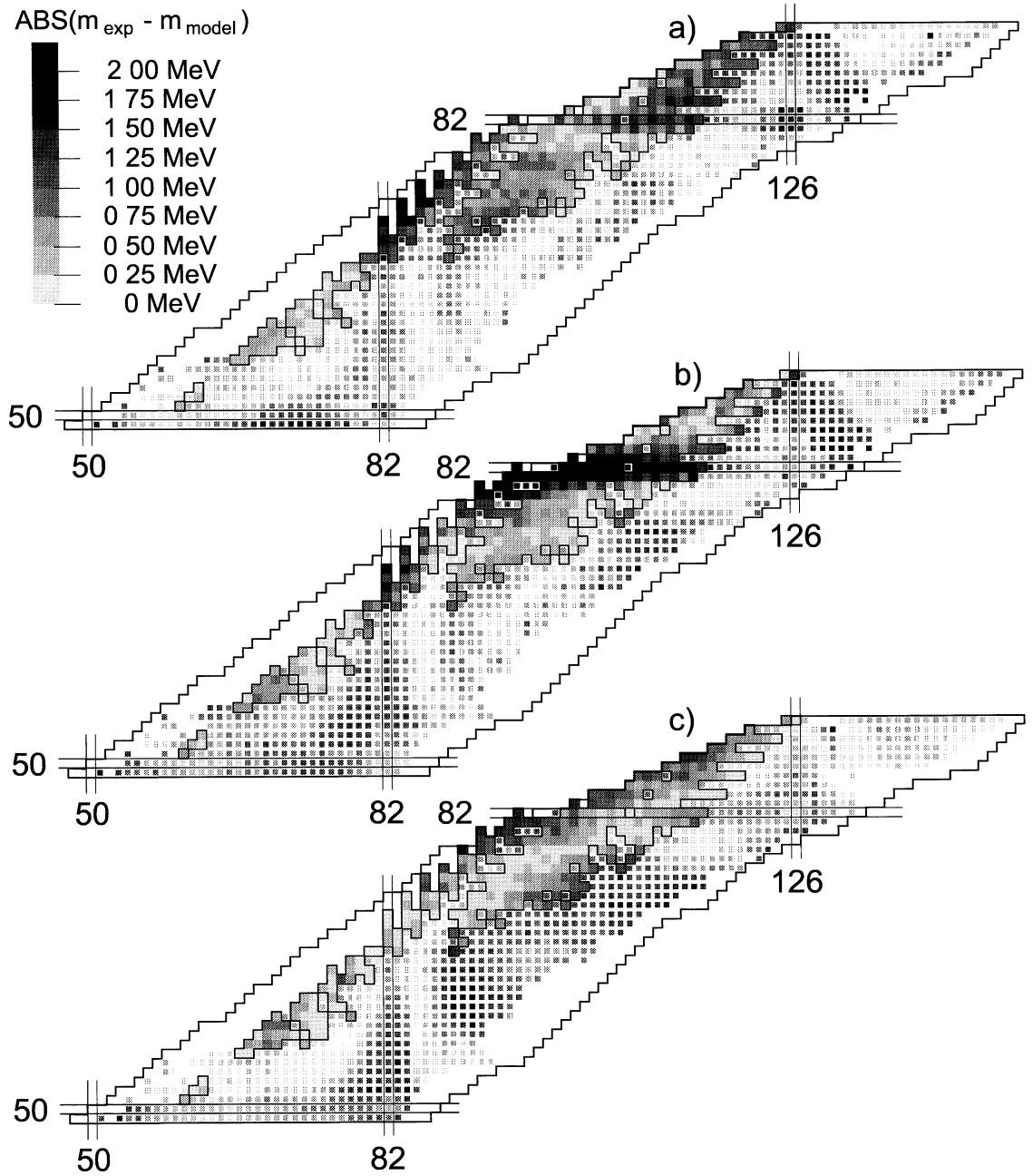
Figure 3 Measured masses compared with models Absolute deviations of measured masses from the HFB (a), HF+BCS (b) and FRDM (c) models are illustrated on the chart of nuclides The large squares represent the new masses with respect to the last AME [8] The comparison yields \sigma_{rms} values of 650, 960 and 372 keV, for the HFB[10], HF+BCS[10] and FRDM[11] models
