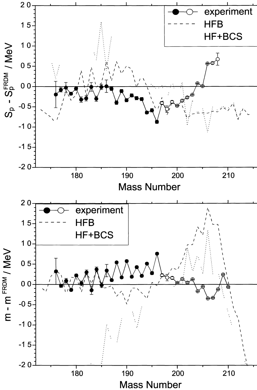
Figure 2 Proton separation energies (upper panel) and mass values (lower panel) of Tl isotopes compared with the HFB [10], HF+BCS[10] and FRDM[11] mass models. The full circles represent our new mass values.
