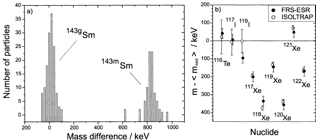
Figure 1. Illustration of the improved accuracy and resolution of SMS. a) The mass spectra analyzed from single ^{143}\text{Sm} ions in the ground and isomeric states. A resolving power of 2 \times 10^6 (FWHM) has been achieved [6,7] by tracing down to single particles. The origin of the horizontal axis represents the corresponding value of AME [8]. b) The measured data from our SMS experiment and from ISOLTRAP [9] are both compared with the prediction of the AME table [8].
