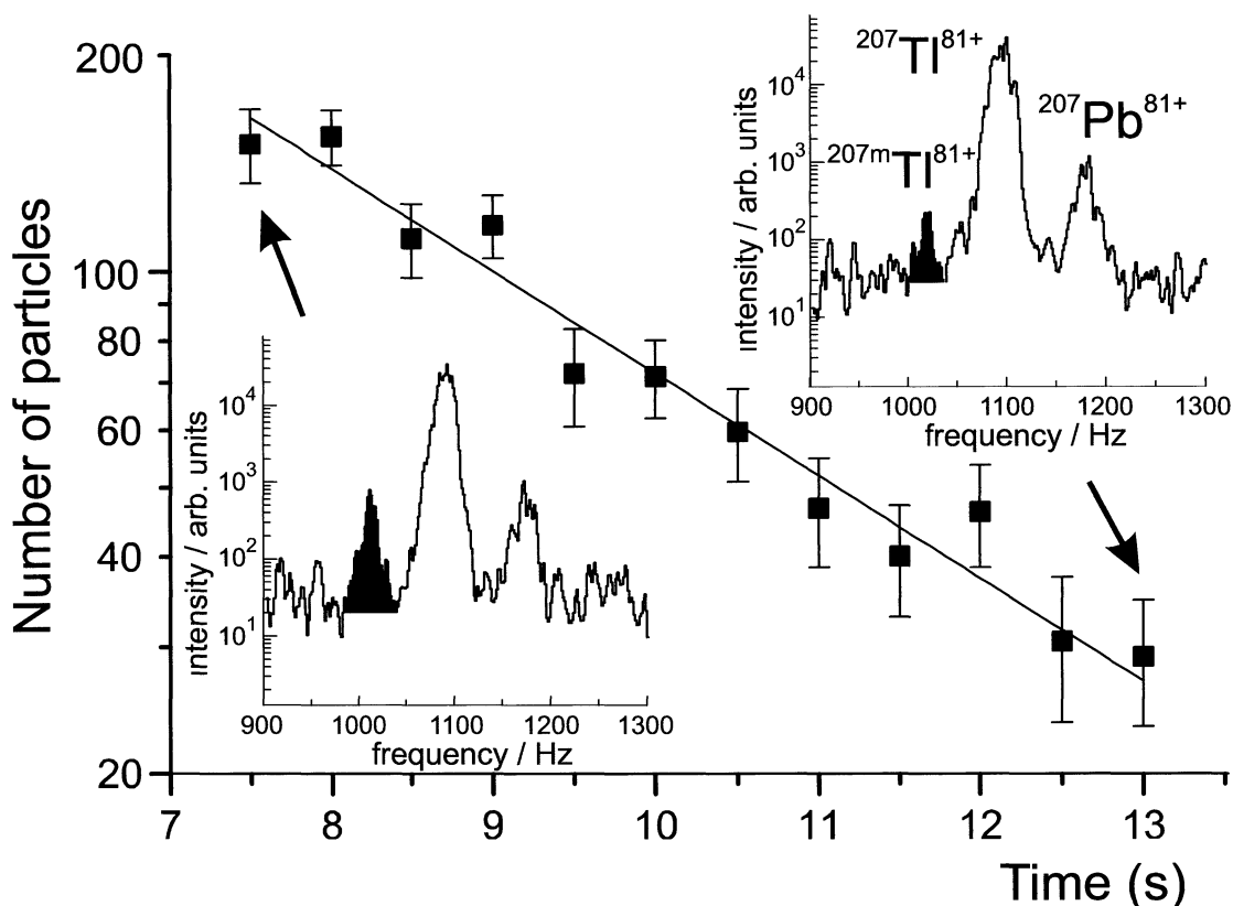
Figure 6 Schottky frequency spectra of the decay of ^{207m}\text{Tl}^{81+} fragments and the corresponding decay curve. The area of the peak in the Schottky spectra is proportional to the number of stored ions. The combination of stochastic and electron cooling yields access to short-lived ions.
