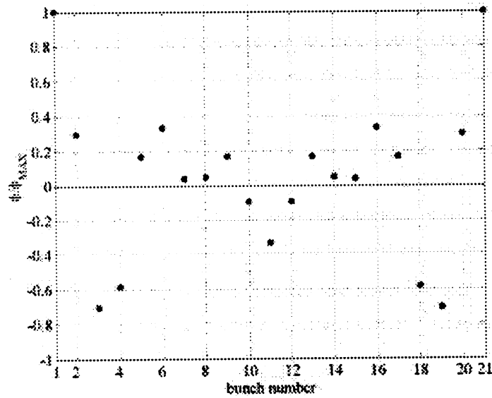
Figure 10 - Deflection of the bunches with 3 close RF frequencies and P_{RF}=9 MW ( \Delta\phi/\phi_{MAX} = 66\% )
