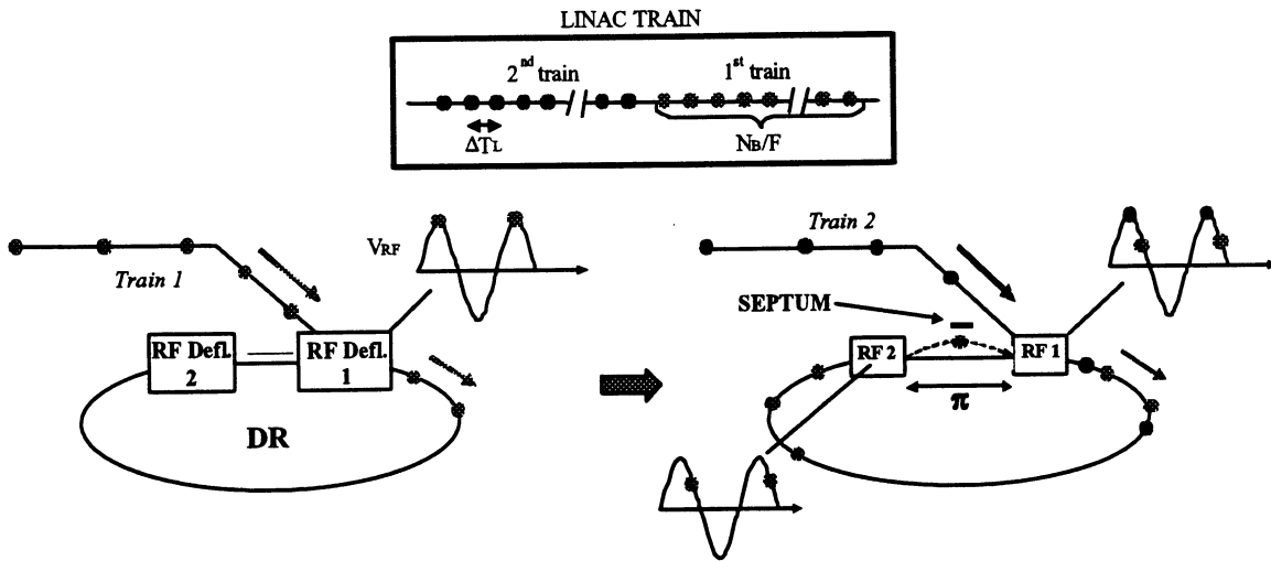
Figure 3 - CTF3-like injection scheme for the TESLA DR
