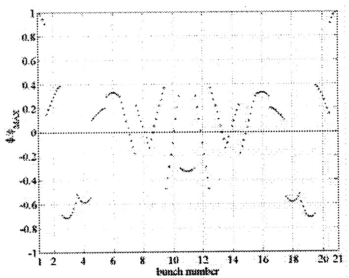
Figure 16 - Deflection of the bunches with 3 distant RF frequencies ( \Delta\phi_{TAIL} / \phi_{MAX} = 57\% ) for a gaussian bunch distribution ( \sigma_z = 6mm )
