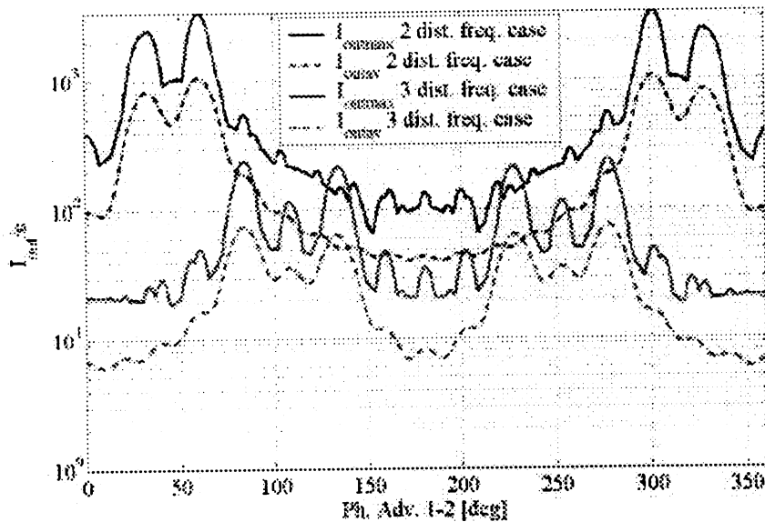
Figure 25 - Average and maximum values of the ratio I_{out}/\epsilon as a function of Ph. Adv. 1-2 and with Ph. Adv. 2-1=179°
