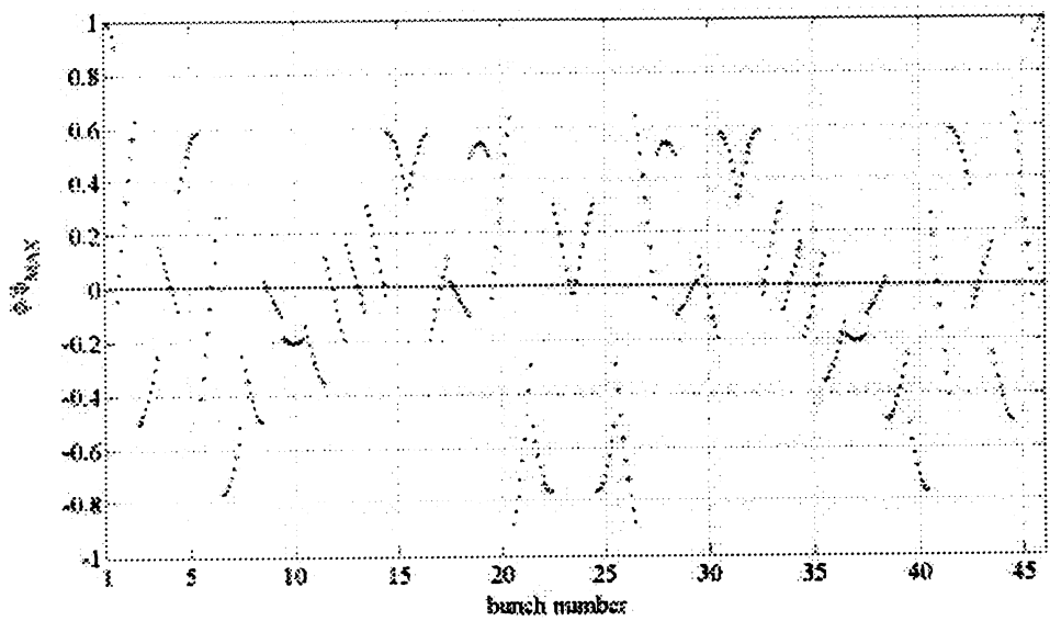
Figure 20 - Deflection of the bunches with 3 distant RF frequencies for a gaussian bunch distribution with \sigma_z = 6mm and F=45 ( \Delta\phi_{TAIL} / \phi_{MAX} = 30\% )
