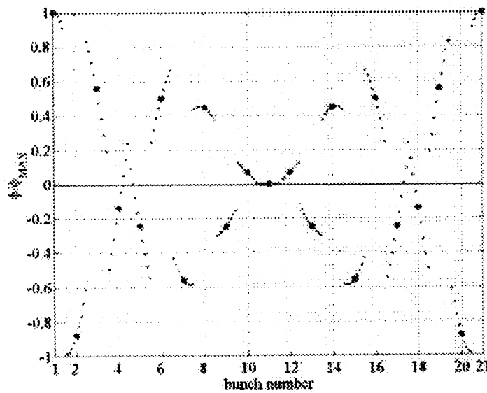
Figure 13 - Deflection of the bunches with 2 RF frequencies (optimized in the macroparticle case) for a gaussian bunch distribution ( \sigma_z = 6mm )
