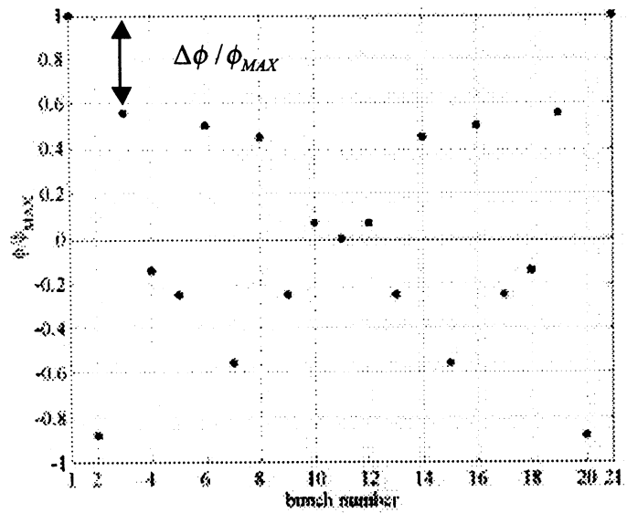
Figure 7 - Deflection of the bunches with 2 RF frequencies ( \Delta\phi/\phi_{MAX} = 44\% )
