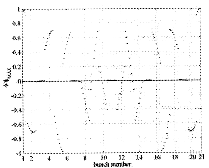
Figure 14 - Deflection of the bunches with 2 distant RF frequencies ( \Delta\phi_{TAIL} / \phi_{MAX} = 22\% ) for a gaussian bunch distribution ( \sigma_z = 6mm )
