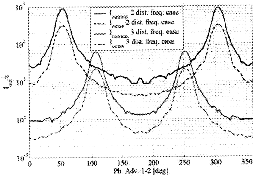
Figure 28 - Average and maximum values of the ratio I_{out}/\epsilon as a function of Ph. Adv. 1-2 with an amplitude variation of +1% of the deflecting voltage RF1 related to f_{RF1}
