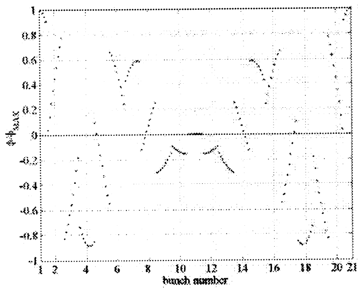
Figure 15 - Deflection of the bunches with 2 close RF frequencies ( \Delta\phi_{TAIL} / \phi_{MAX} = 14\% ) for a gaussian bunch distribution ( \sigma_z = 6mm )
