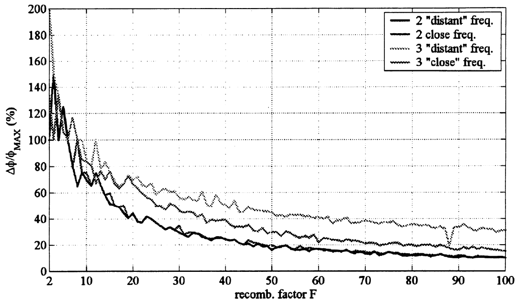
Figure 11 - \Delta\phi / \phi_{MAX} considering different recombination factor F
