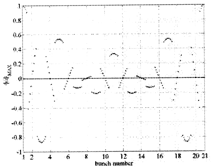
Figure 17 - Deflection of the bunches with 3 close RF frequencies ( \Delta\phi_{TAIL} / \phi_{MAX} = 38\% ) for a gaussian bunch distribution ( \sigma_z = 6mm )
