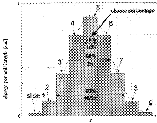
Figure 12 - Discretized gaussian bunch profile
