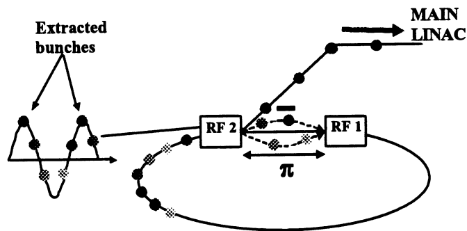
Figure 4 - CTF3-like extraction scheme for the TESLA DR
