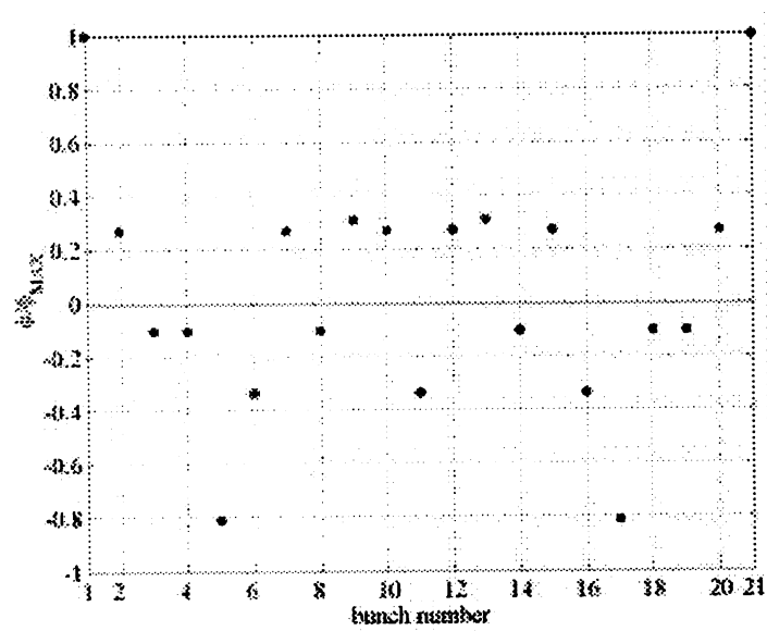
Figure 9 - Deflection of the bunches with 3 distant RF frequencies ( \Delta\phi/\phi_{MAX} = 69\% )
