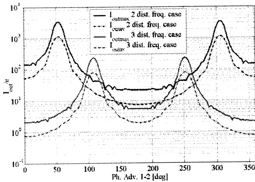
Figure 29 - Average and maximum values of the ratio I_{out}/\epsilon as a function of Ph. Adv. 1-2 with a phase variation of +1% of the deflecting voltage RF1 related to f_{RF1}
