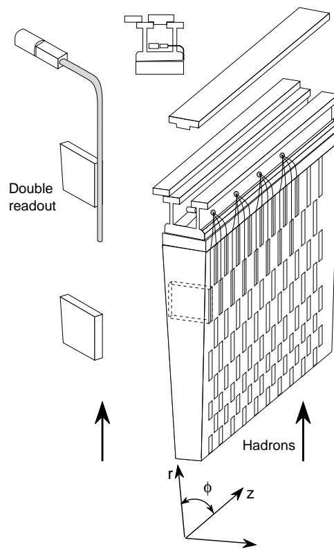
Figure 1: Principle of the tile hadronic calorimeter.
