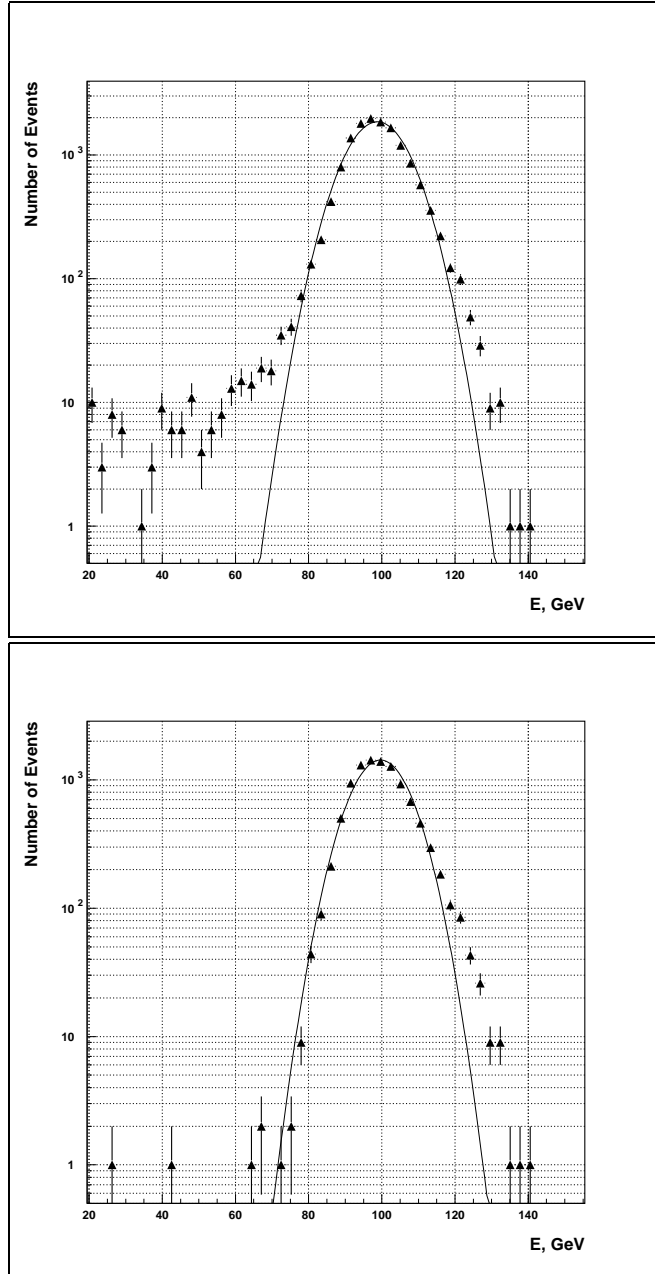
Figure 7: Energy responses for all Z = -8 \text{ cm} at a different leakage conditions: all events (top), no leakage (bottom).
