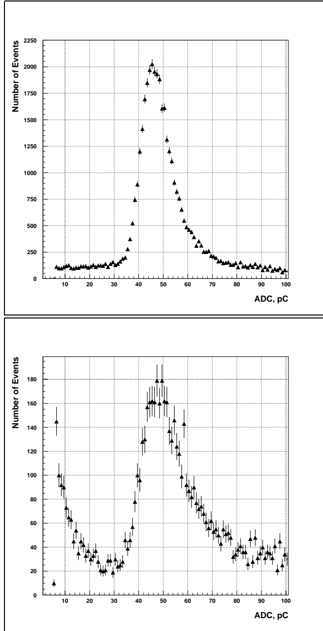
Figure 2: Typical ADC spectrum of a “muon wall” counters in the \mu beam (top) and in the \pi beam (bottom) for counter N^{\circ} 8 .
