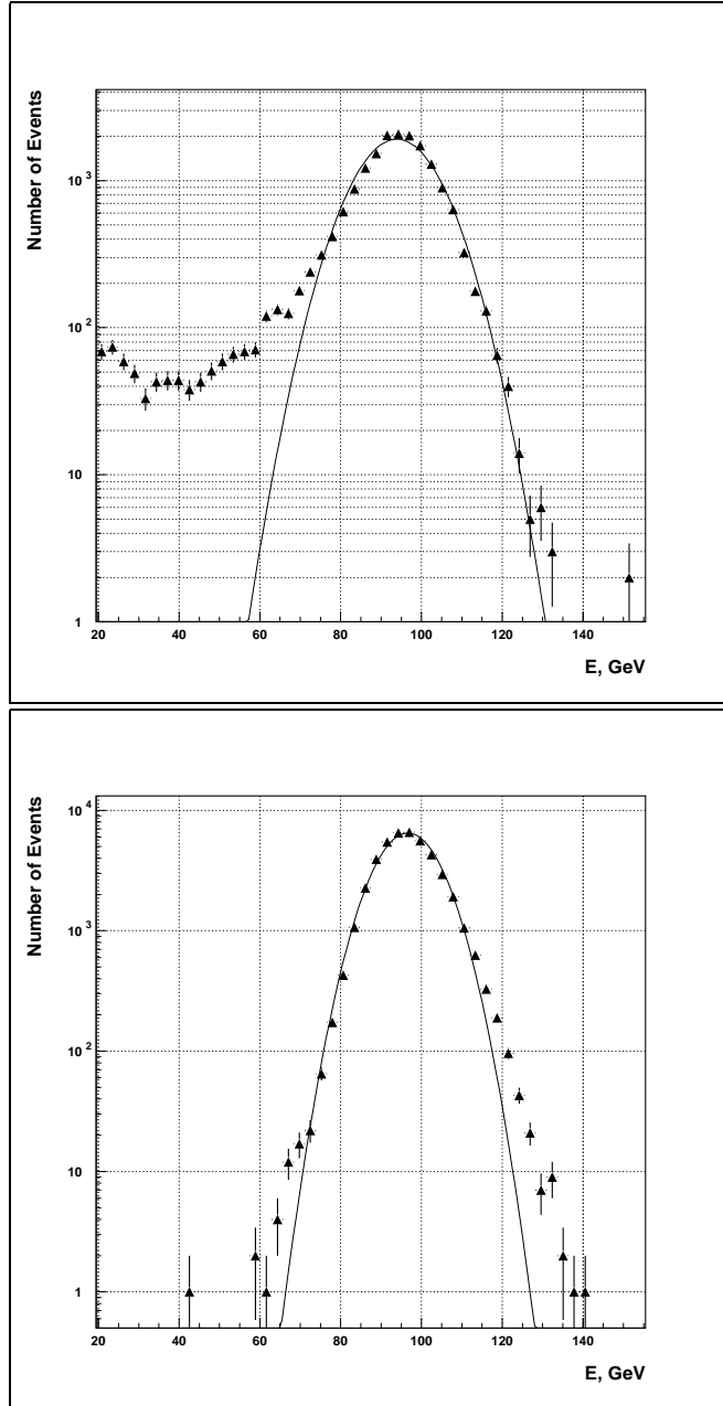
Figure 6: Energy responses for Z at a different leakage conditions: longitudinal leakage (top), lateral leakage (bottom).
