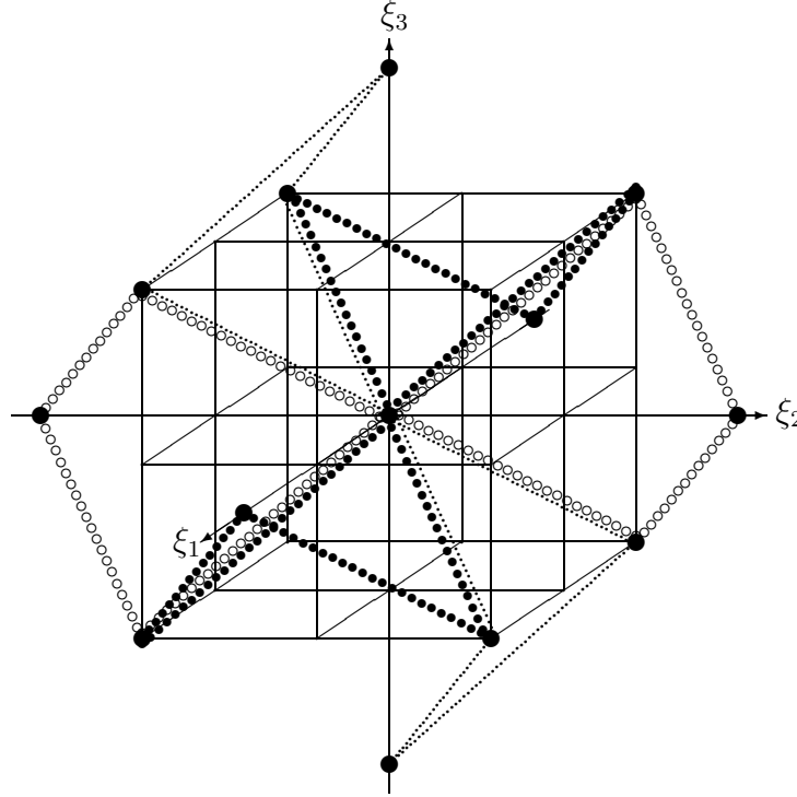
Figure 6.2: The six faces of the polyhedron Q(1, 1) containing o .
