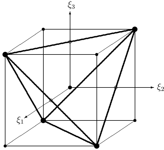
Figure 4.1: A regular tetrahedron inscribed in a cube.
