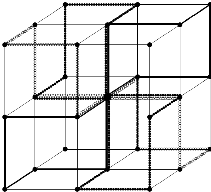
Figure 5.2: The six faces of the polyhedron P(1,0) containing o .
