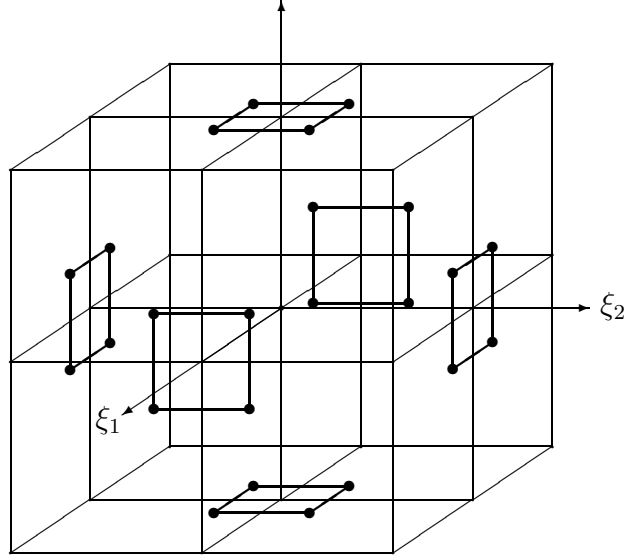
Figure 6.3: The points of W for c = 1 and d = 4 .
