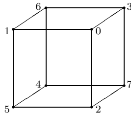
Figure 6.1: The cube representing the action of H_0 .
