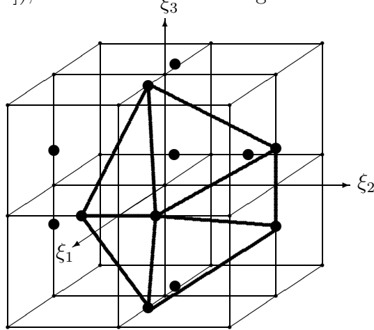
Figure 5.1: The points of V for a = 1 and b = 3 .
