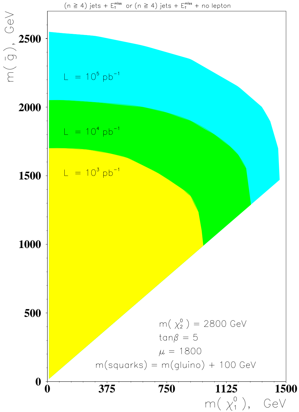
Figure 2: CMS discovery potential for different values of m_{\tilde{\chi}_1^0} and m_{\tilde{g}} in the case of m_{\tilde{g}} > m_{\tilde{\chi}_1^0}
