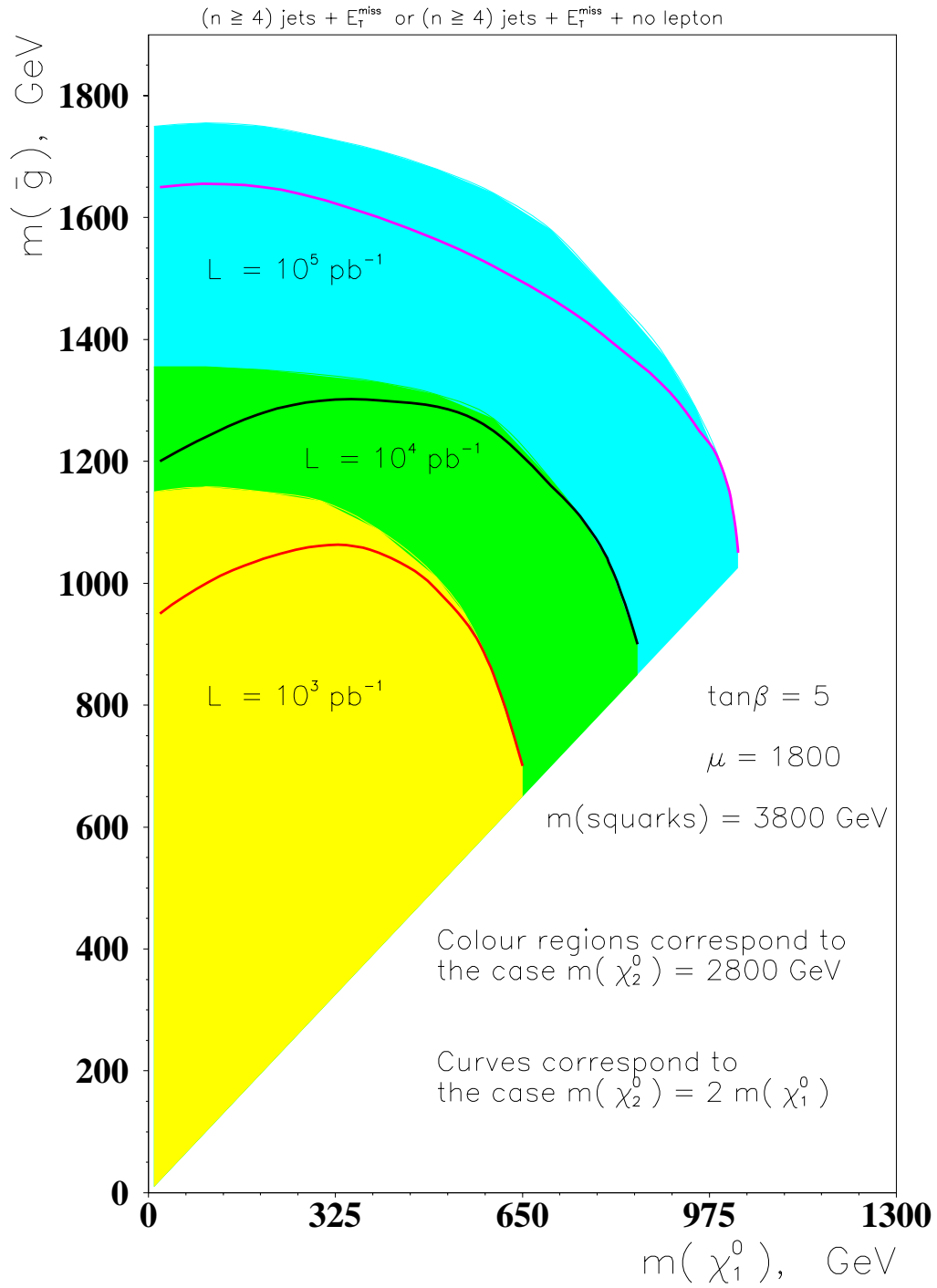
Figure 1: CMS discovery potential for different values of m_{\tilde{\chi}_1^0} and m_{\tilde{g}} in the case of m_{\tilde{g}} > m_{\tilde{\chi}_1^0} .
