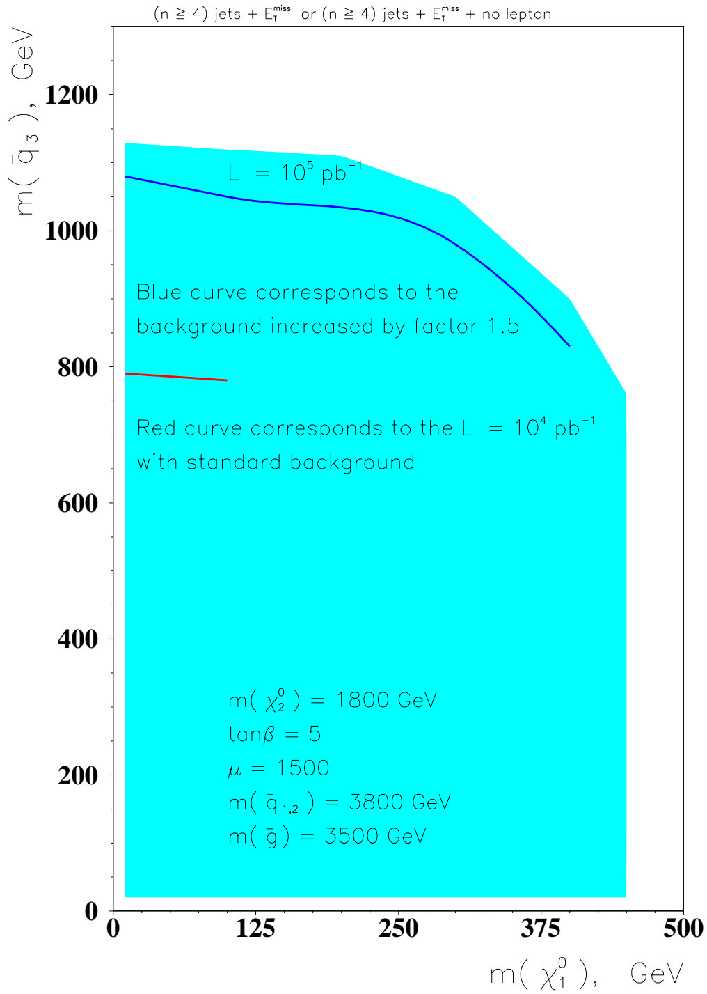
Figure 4: CMS discovery potential for different values of m_{\tilde{\chi}_1^0} and m_{\tilde{q}_3} in the case of m_{\tilde{q}_{1,2}} \gg m_{\tilde{q}_3} .
