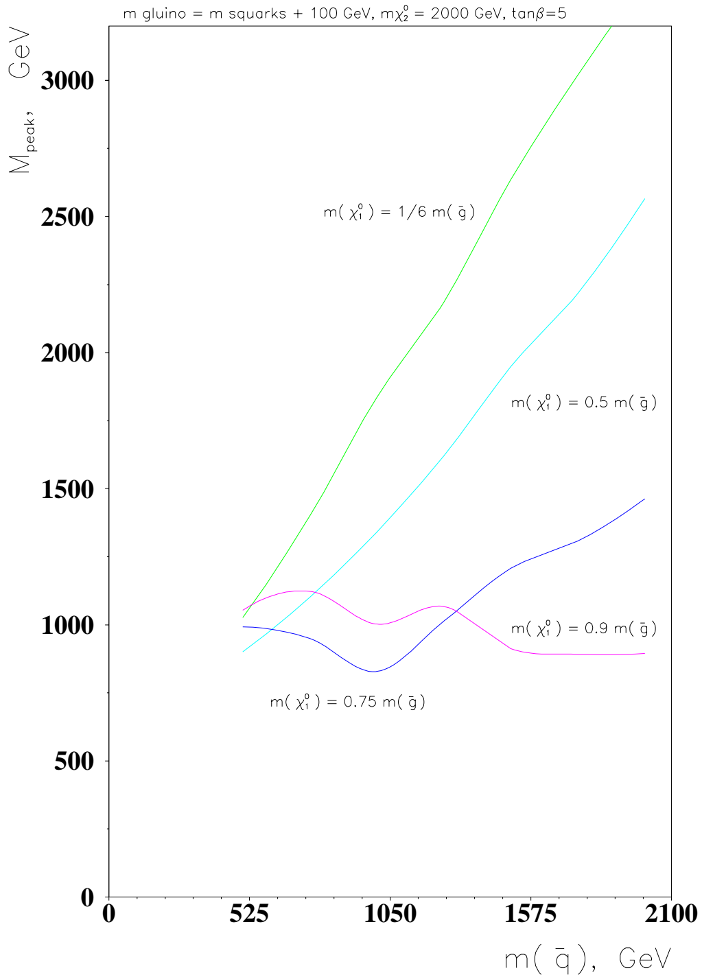
Figure 8: The dependence of the M_{susy} \equiv M_{peak} on the squark mass for different values of m(\chi_1^0) .
