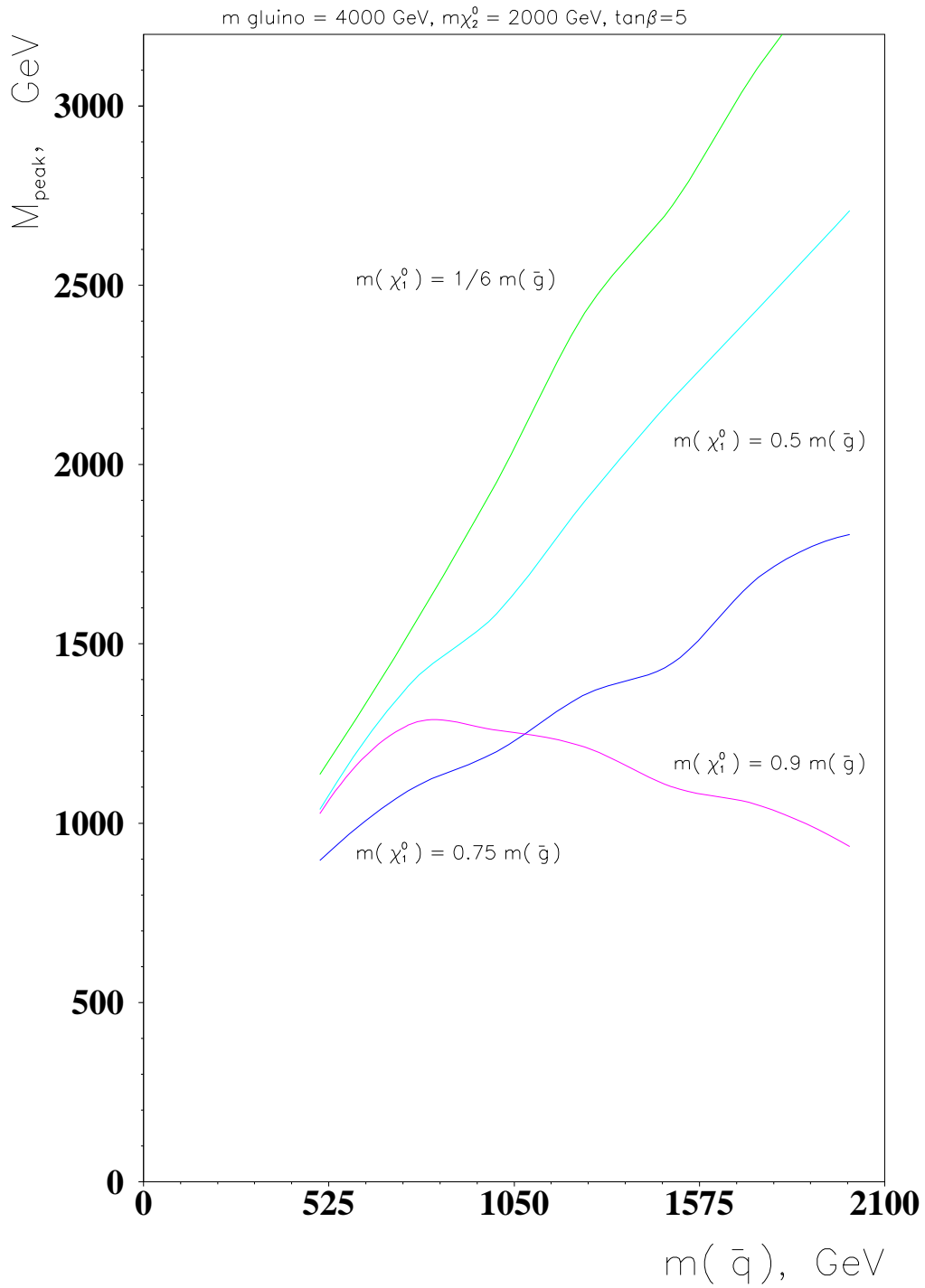
Figure 7: The dependence of M_{\text{susy}} \equiv M_{\text{peak}} on the squark mass for different values of m(\chi_1^0) .
