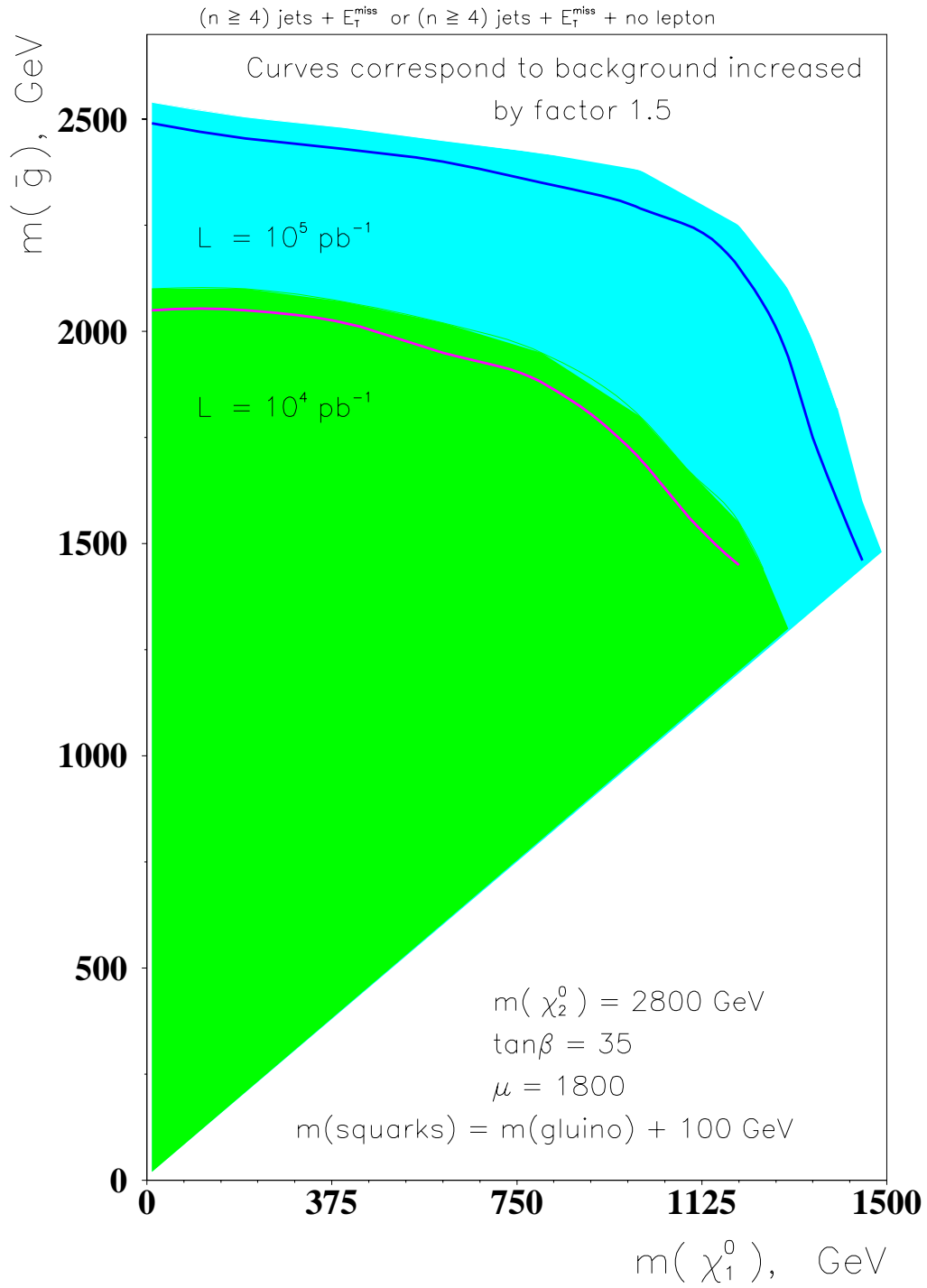
Figure 3: CMS discovery potential for different values of m_{\tilde{\chi}_1^0} and m_{\tilde{g}} in the case of m_{\tilde{g}} > m_{\tilde{\chi}_1^0} .
