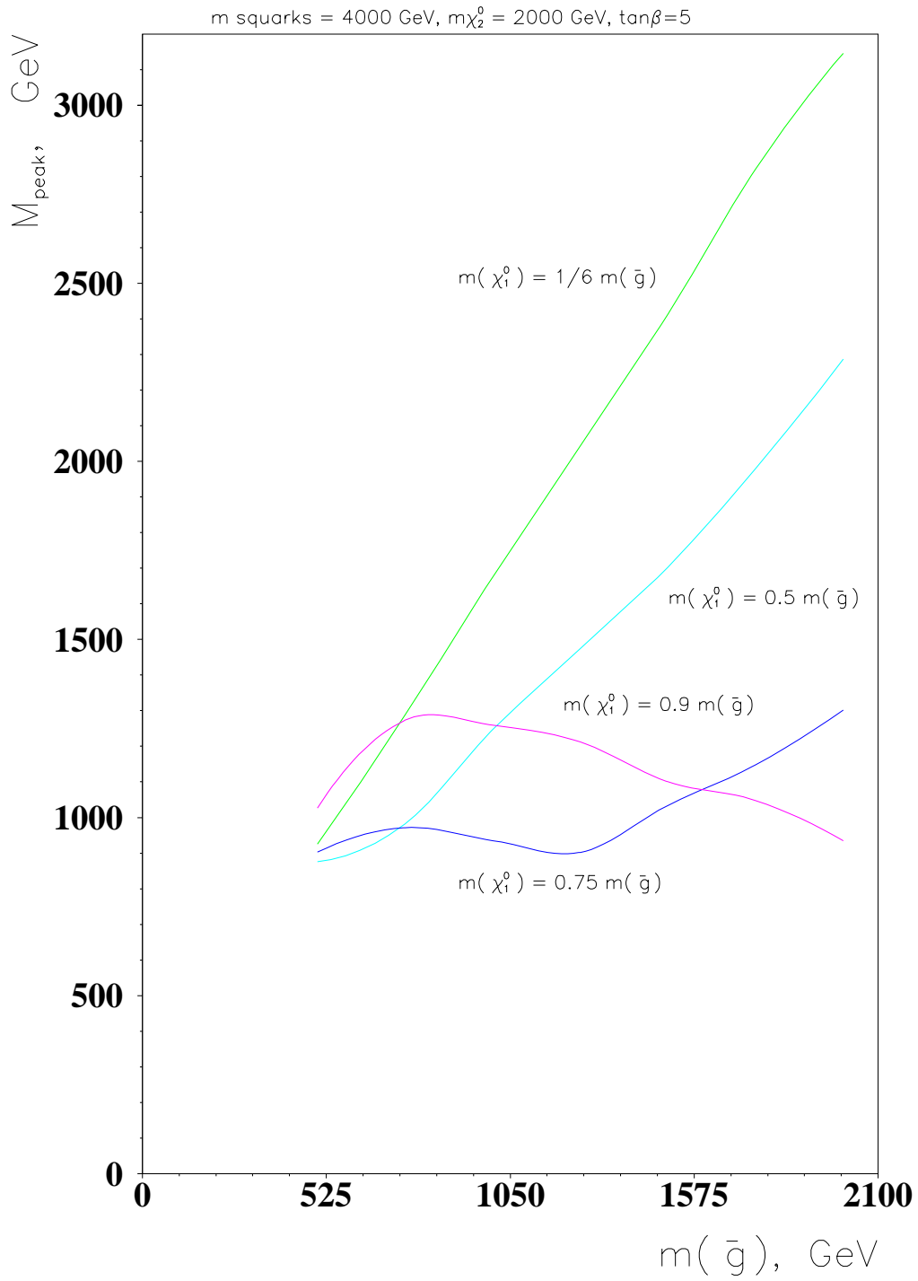
Figure 6: The dependence of M_{susy} \equiv M_{peak} on the gluino mass for different values of m(\chi_1^0) .
