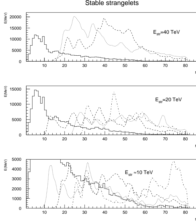
Figure 11. Transition curves of stable strangelets with energy E_{str} = 10\text{-}40 TeV, baryon number A_{str} = 15\text{-}40 , quark chemical potential \mu_q = 600, 1000 MeV. Energy deposit (MeV) in the calorimeter layers, in the octant containing a strangelet, is shown. Full line histograms show the HIJING estimated background.
