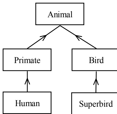
Figure 7: Normal Class Hierarchy for Humans and Superbirds
