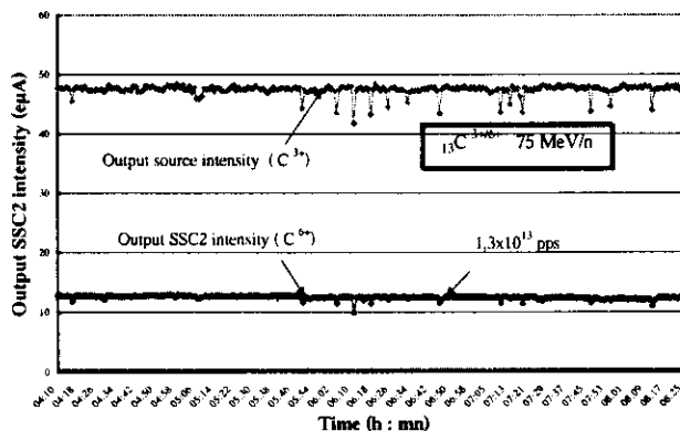
Figure 2 : Source and SSC2 output intensities versus time for the carbon beam
