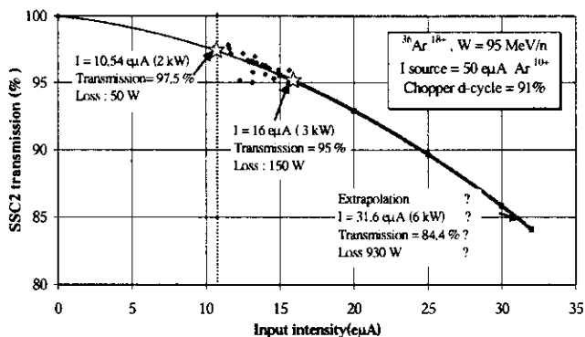
Fig.1 : SSC2 transmission efficiency versus input intensity for an argon beam.
