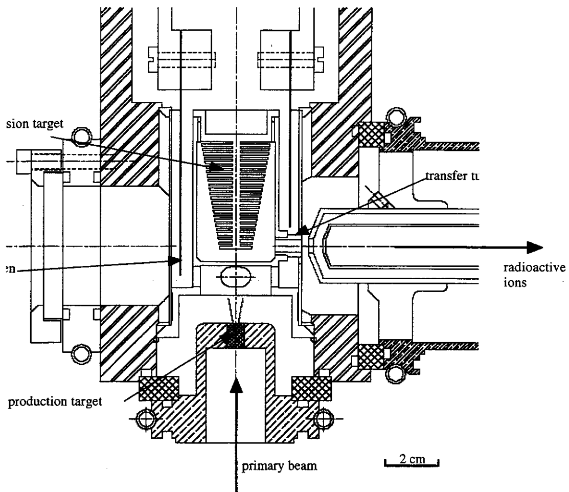
Figure 3: The monolithic configuration where the transfer tube is the surface ionizer
