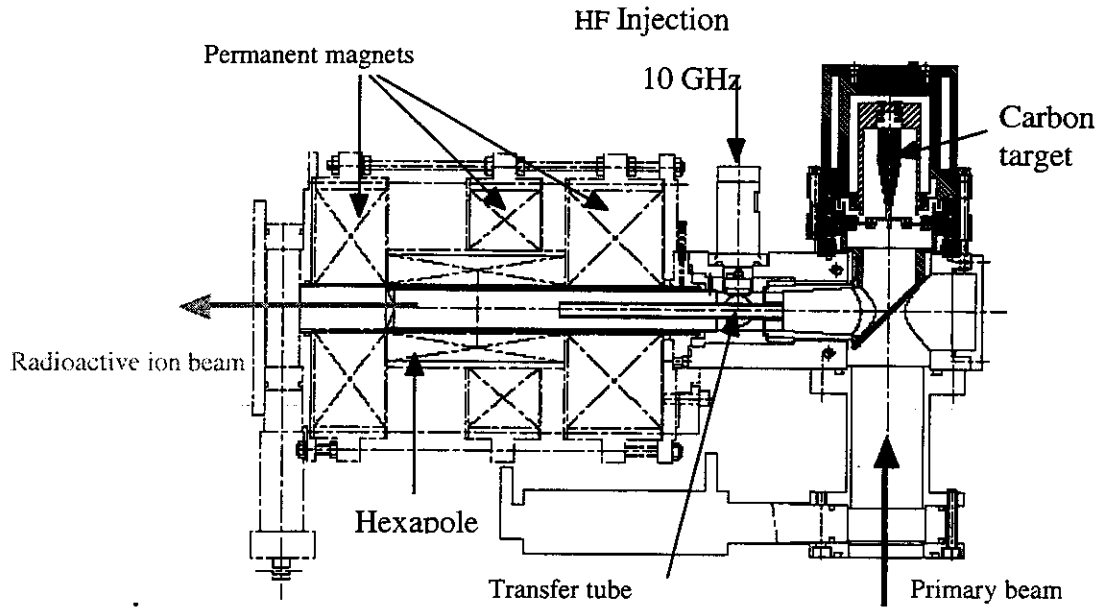
. Figure 1: The nanogan3 configuration: a permanent magnet ECRIS is coupled to a graphite target through a cold transfer tube
