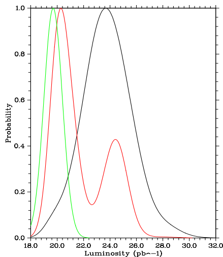
Figure 13. Probability distribution of the luminosity (run1a in pb^{-1} ) for the unit-weighted (right plot) and weighted (middle plot) PDFs, compared to the value used by CDF (left plot).
