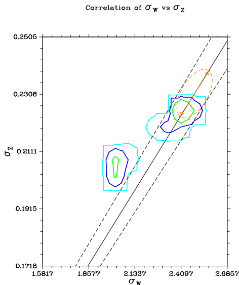
Figure 12. Same as in Fig. 10 for the weighted PDFs.
