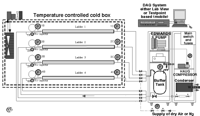
Figure 1: The Two-Stage Evaporative Recirculator
