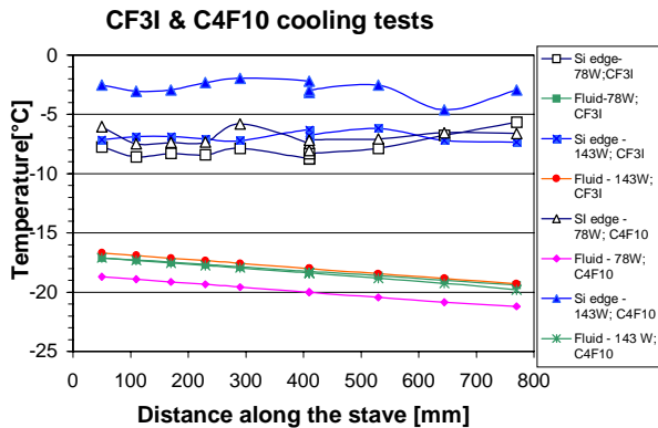
Figure 11a: Temperature Profiles along the Pixel C-C stave: CF 3 I and C 4 F 10
