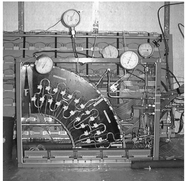
Figure 2: Forward SCT Quadrant Thermal Model
