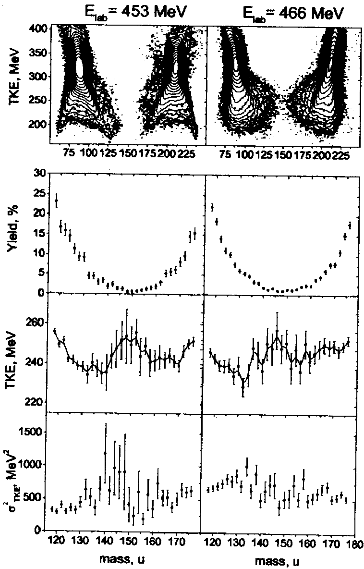
Figure 5: Mass-energy distributions of the ^{86}\text{Kr}+^{208}\text{Pb} reaction products.
