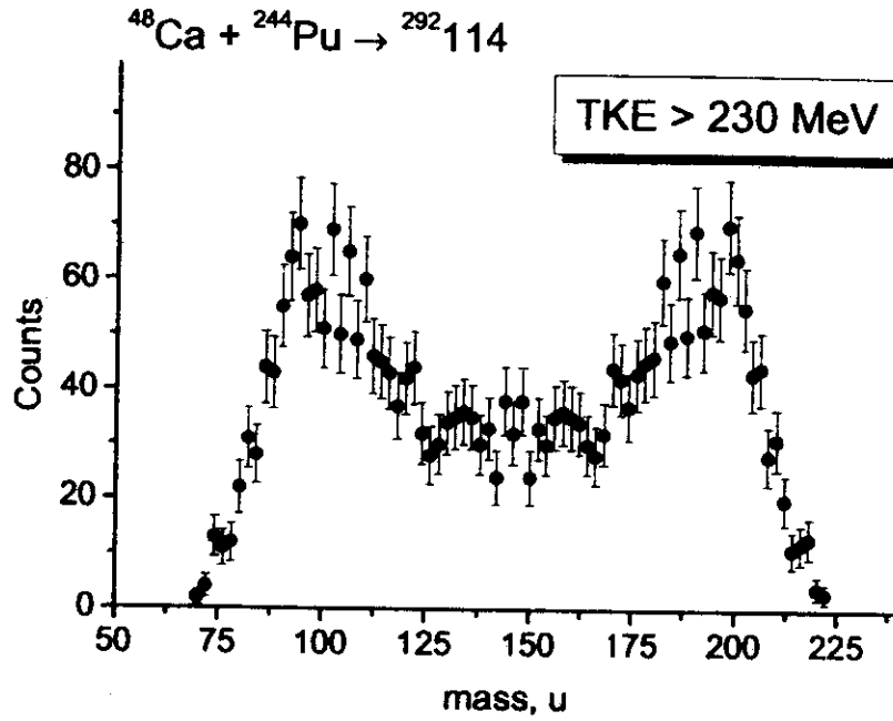
Figure 4: Fission fragment mass distribution for the ^{48}\text{Ca}+^{244}\text{Pu} reaction for the range of \text{TKE} > 230 MeV.
