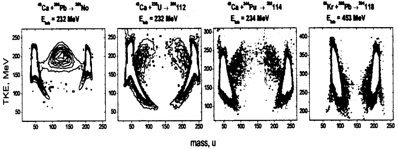
Figure 1: Two-dimensional matrices TKE–Mass of the products of the indicated reactions.
