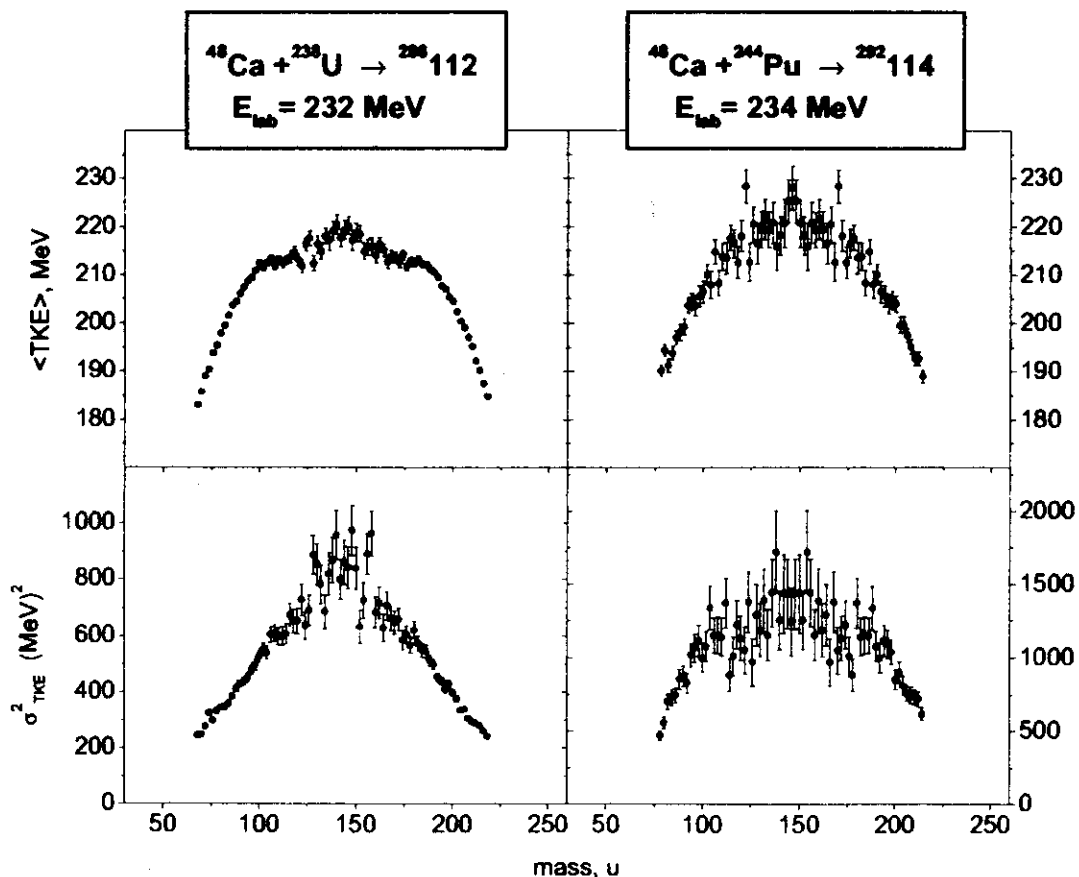
Figure 3: TKE and \sigma_{\text{TKE}}^2 distributions in dependence on the fragment mass for the same reactions as in Fig.2.
