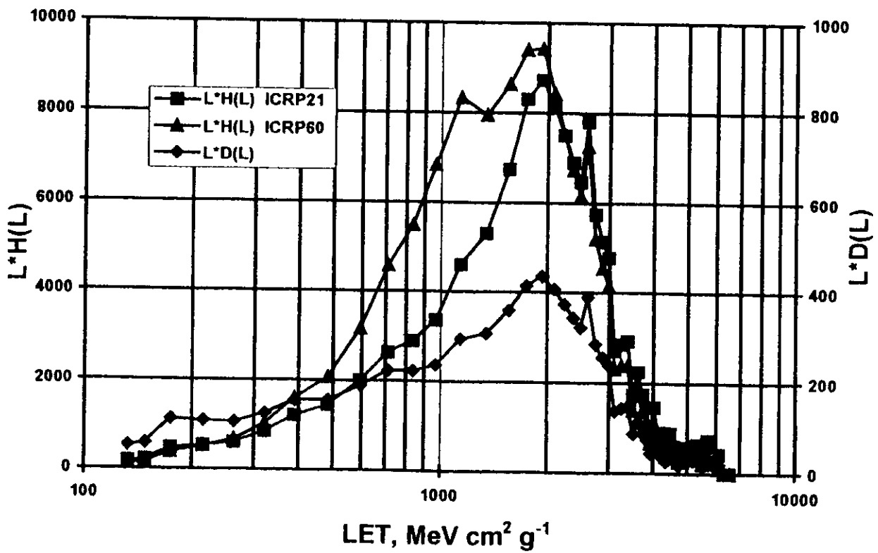
Fig.3. Microdosimetric distributions of the absorbed and equivalent doses due to the secondary particles in the 1 GeV proton beam
