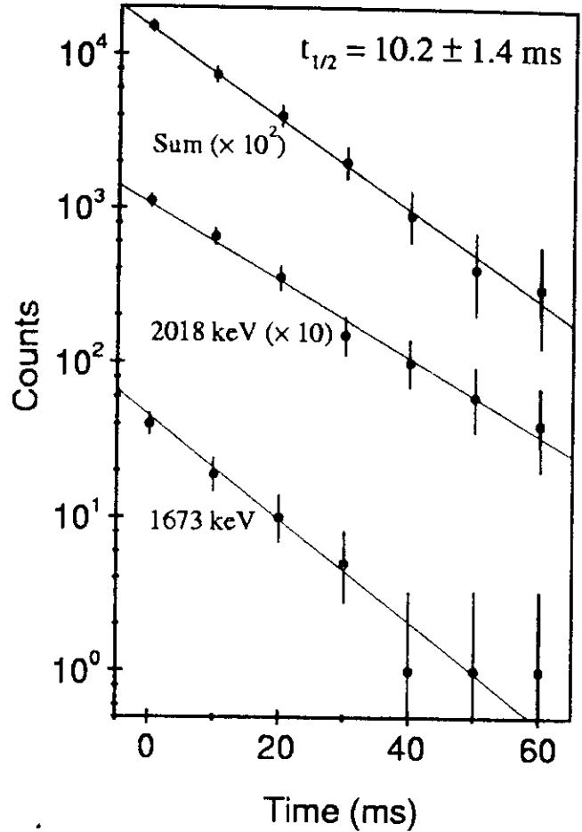
Fig. 6. Decay curves for the two \gamma -ray transitions assigned to the \beta -decay of ^{26}\text{F} to levels in ^{26}\text{Ne} and the sum of these data. Each data set is plotted with the appropriate result of a maximum likelihood fit.
