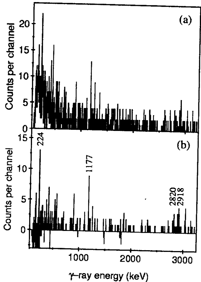
Fig. 11. Energy spectra of a) all \beta -delayed \gamma -rays occurring within 50 ms of the arrival of a ^{29}\text{Ne} ion at the focal plane of LISE3; b) the same spectrum after the subtraction of a normalised fraction of the background spectrum. The \gamma -rays associated with the \beta -decay of ^{29}\text{Ne} are labelled with their energy in keV.
