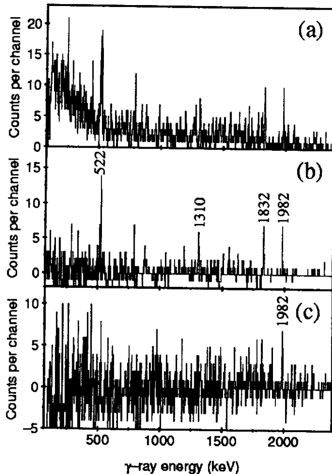
Fig.1. Energy spectra of a) all \beta -delayed \gamma -rays occurring within 200 ms of the implantation of a ^{24}\text{O} ion; b) the same spectrum following the subtraction of the background spectrum observed at this setting of the LISE3 spectrometer; and c) the background subtracted energy spectrum of \beta -delayed \gamma -rays occurring between 200 ms and 1 s after the arrival of a ^{24}\text{O} ion. \gamma -ray peaks associated with the \beta -decay of ^{24}\text{O} and its daughter ^{24}\text{F} are labelled according to their energy in keV.
