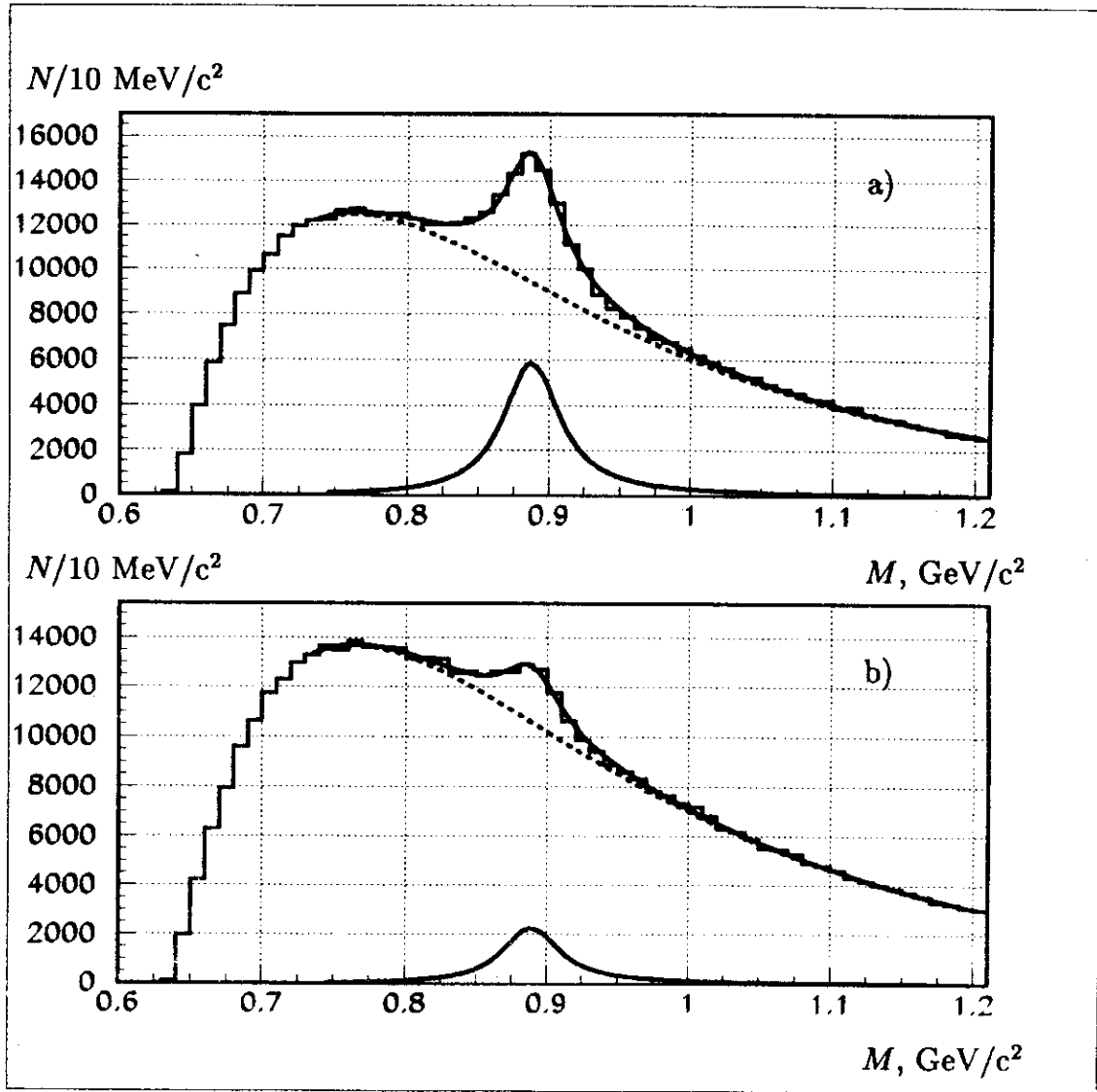
Fig. 1. Invariant mass spectra of K_S \pi^+ (a) и K_S \pi^- (b) combinations; the dashed curve represents the background; the shaded spectrum shows the signal contribution.
