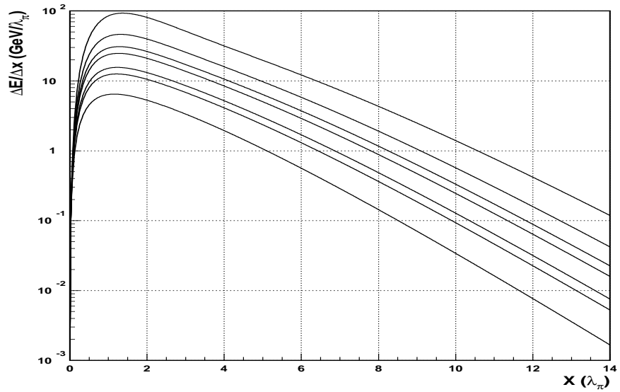
Figure 6: The calculated differential longitudinal energy deposition, dE/dx , as a function of the longitudinal coordinate x in units \lambda_\pi for the LAr (top) and Tile (bottom) calorimeters at 20 – 300 GeV.
