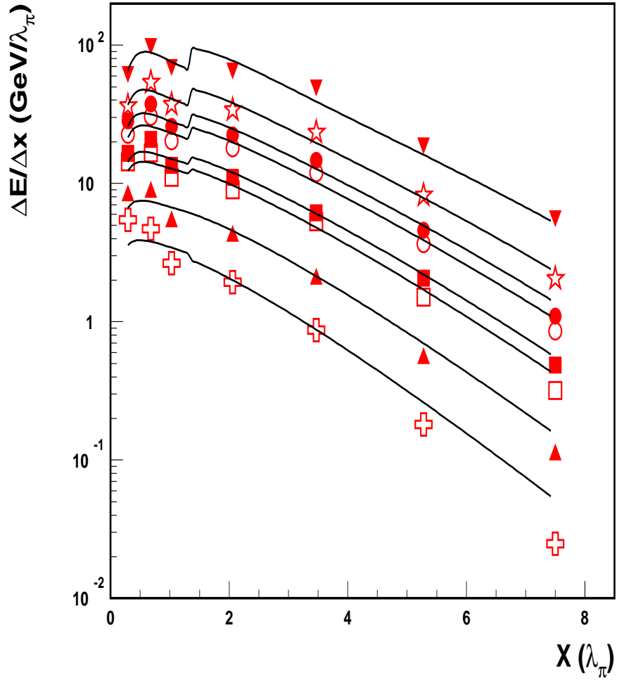
Figure 9: The experimental differential longitudinal energy depositions at 10 GeV (crosses), 20 GeV (black top triangles), 40 GeV (open squares), 50 GeV (black squares), 80 GeV (open circles), 100 GeV (black circles), 150 GeV (stars), 300 GeV (black bottom triangles) energies as a function of the longitudinal coordinate x in units \lambda_\pi for the combined calorimeter and the results of the description by the modified parameterization.
