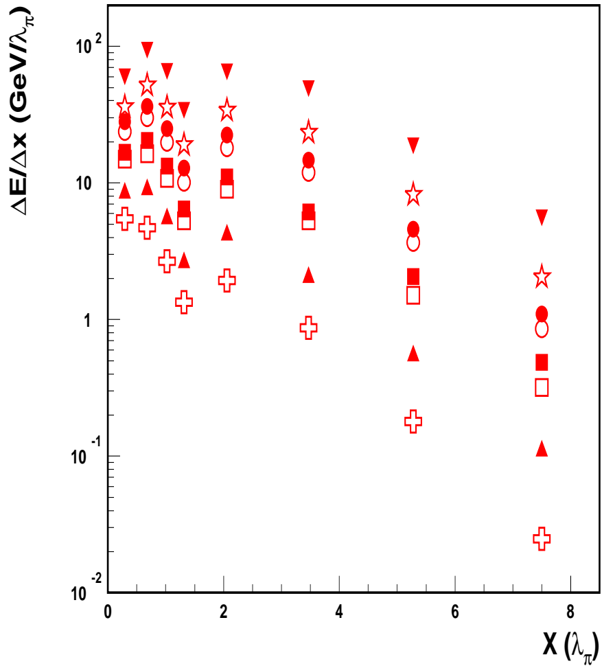
Figure 4: The differential longitudinal energy depositions in each longitudinal sampling for 10 GeV (crosses), 20 GeV (black top triangles), 40 GeV (open squares), 50 GeV (black squares), 80 GeV (open circles), 100 GeV (black circles), 150 GeV (stars) and 300 GeV (black bottom triangles) energies as a function of the longitudinal coordinate x in units \lambda_\pi for combined calorimeter.
