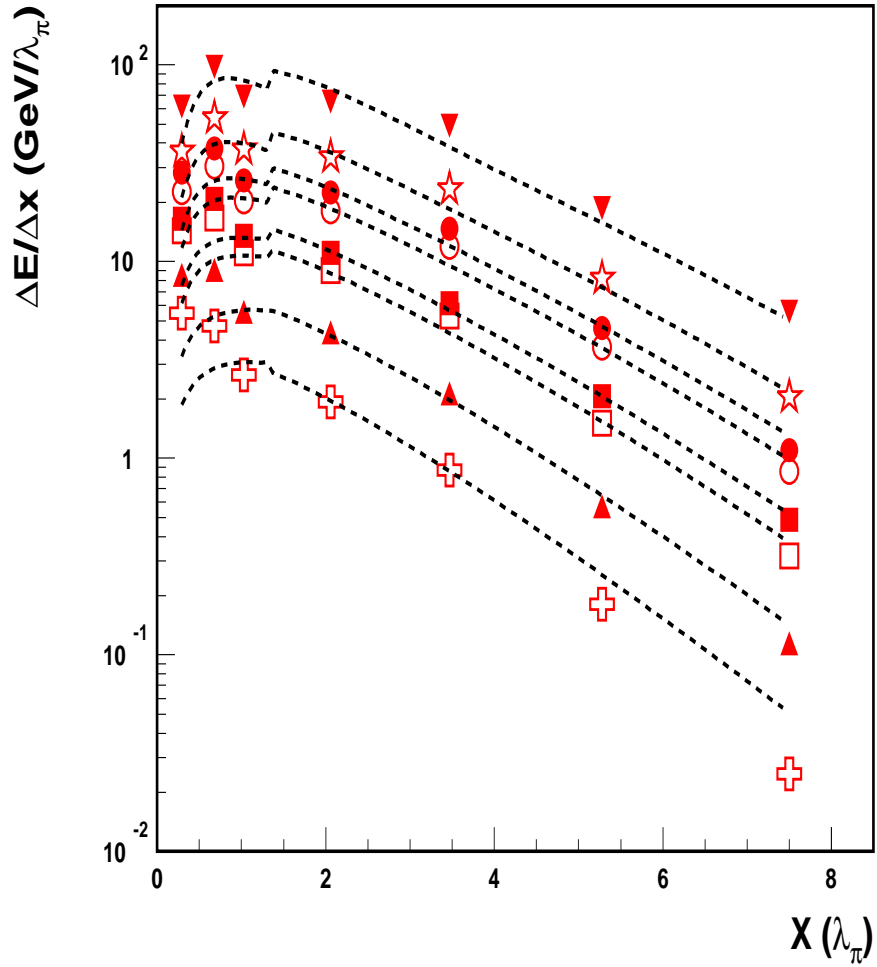
Figure 8: The comparison between the experimental differential energy depositions at 10 GeV (crosses), 20 GeV (black top triangles), 40 GeV (open squares), 50 GeV (black squares), 80 GeV (open circles), 100 GeV (black circles), 150 GeV (stars), 300 GeV (black bottom triangles) and the calculated curves as a function of the longitudinal coordinate x in units \lambda_\pi .
