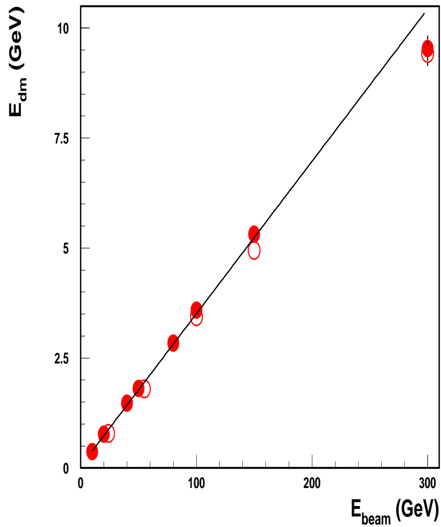
Figure 2: The comparison between the Monte Carlo simulation (open circles) and the calculated values (solid circles).
