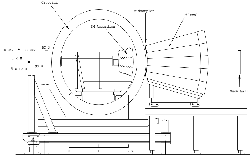
Figure 1: Test beam setup for the combined LAr and Tile calorimeters run.
