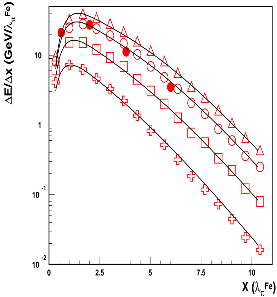
Figure 5: The demonstration of the correctness of the formula (11). The comparison between the calculations by this formula and the experimental data at 20 GeV (crosses), 50 GeV (squares), 100 GeV (open circles), 140 GeV (triangles) energies for conventional iron-scintillator calorimeter [17] and at 100 GeV (black circles) for the Tile calorimeter as a function of the longitudinal coordinate x in units \lambda_{\pi, Fe}
